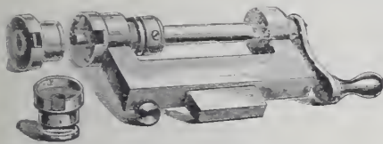
A WATCHMAKER'S WINDING BARREL.
