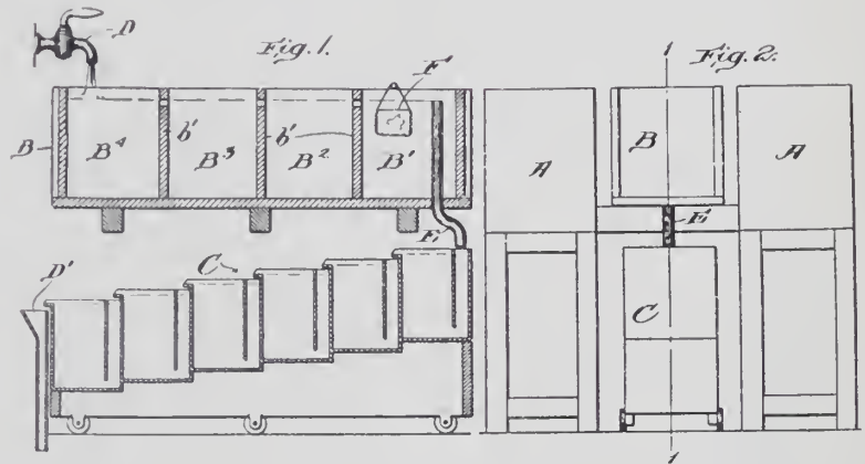
APPARATUS FOR SAVING GOLD FROM RINSE WATER.
