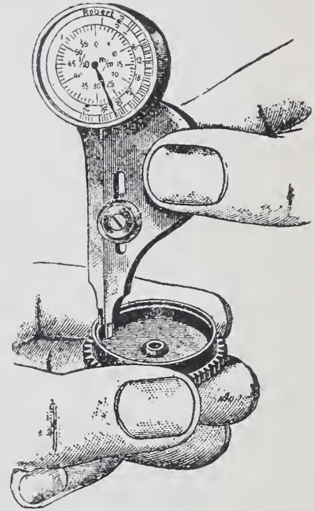
DEVICE FOR MEASURING SPRING'S HEIGHT.
