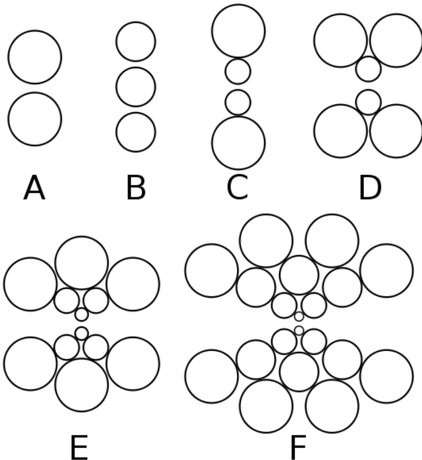
Various rolling configurations. Key: A. 2-high B. 3-high C. 4-high D. 6-high E&F. Cluster
