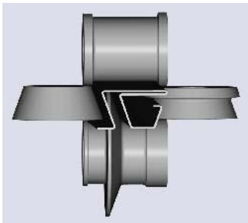
Roll forming
