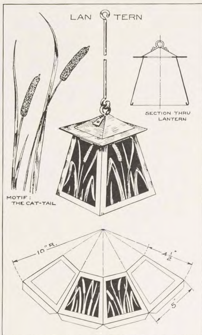
FIG. 123. TRUNCATED PYRAMID SHAPED LANTERN WITH MOTIF FOR THE DESIGN
