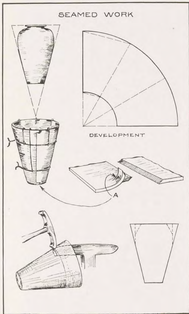
FIG. 148. PREPARATIONS FOR A SEAMED PIECE OF WORK
