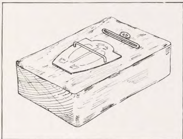
FIG. 21. WORK PREPARED FOR SOLDERING ON THE CHARCOAL BLOCK
