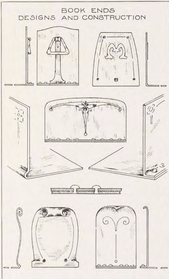
FIG. 110. DESIGNS FOR METAL BOOK ENDS
