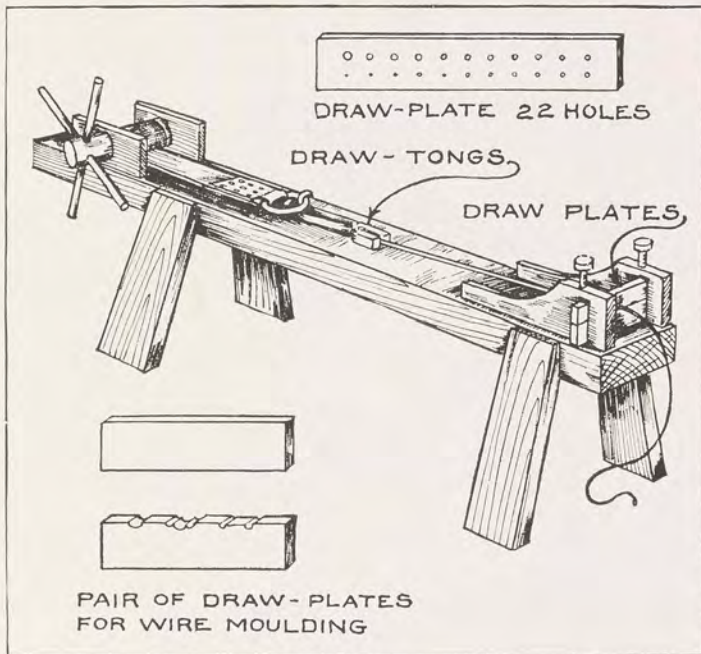
FIG. 90. THE DRAW-BENCH, USED FOR DRAWING HEAVY GAGE WIRE OR MOULDED WIRE
