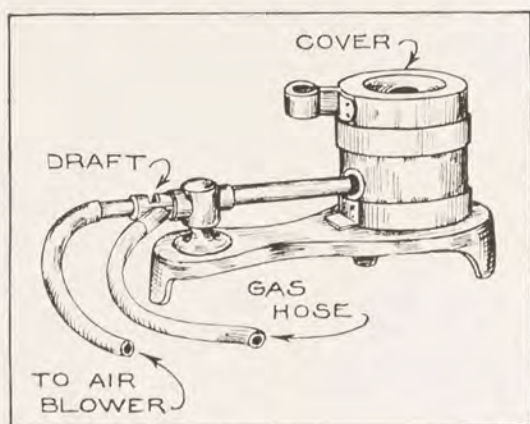
FIG. 105. THE CRUCIBLE FURNACE FOR MELTING SCRAPS OR SMALL QUANTITIES OF METALS
