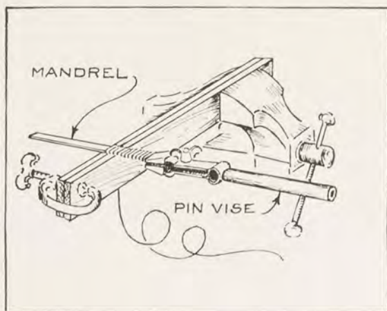
FIG. 91. MAKING LINKS FOR CHAIN WORK
