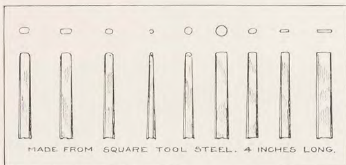
FIG. 52. A FEW USEFUL CHASING TOOLS
