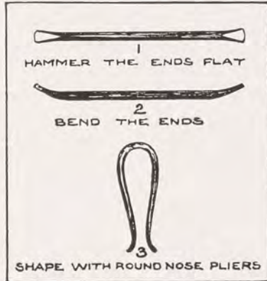
FIG. 25. HOW TO MAKE SMALL IRON CLAMPS
