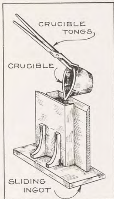
FIG. 106. POURING THE MOULTEN METAL INTO THE INGOT
