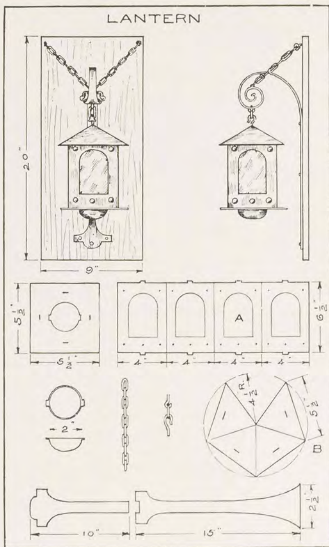
FIG. 121. WALL LANTERN WITH WORKING DRAWINGS
