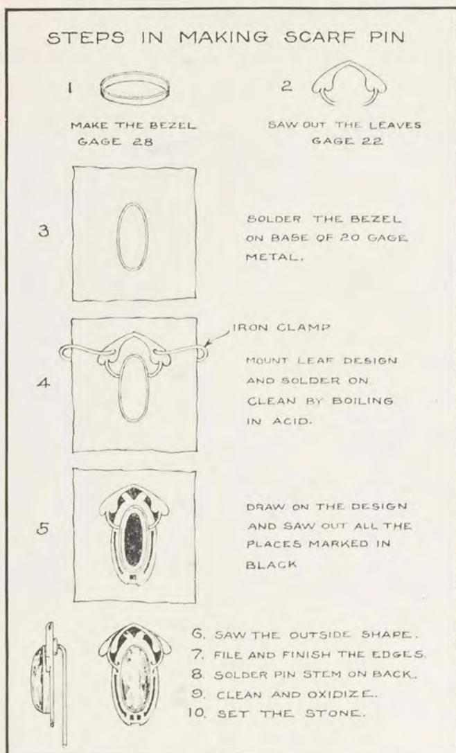
FIG. 57. A SCARF PIN IN THE MAKING
