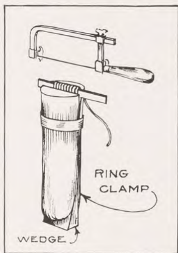
FIG. 92. SAWING THE COILED WIRE LINKS
