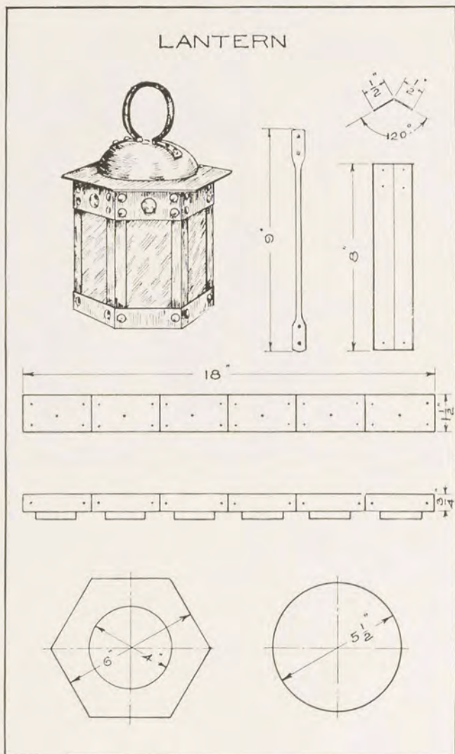
FIG. 125. RIVETED LANTERN, HEXAGONAL SHAPED
