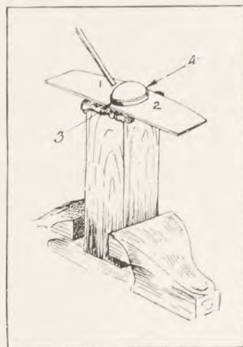
FIG. 42. SETTING A STONE
