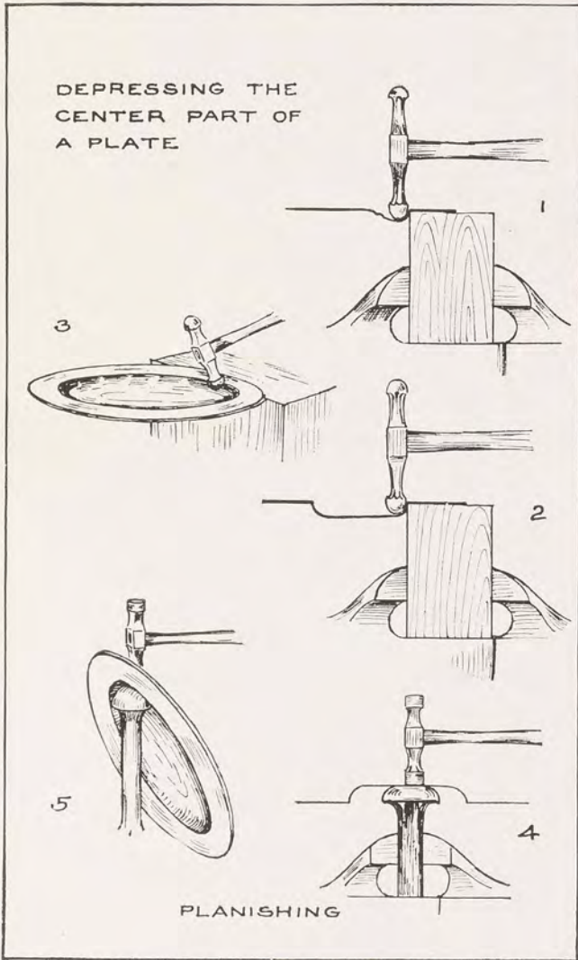
FIG. 146. SUCCESSIVE STEPS IN MAKING A PLATTER
