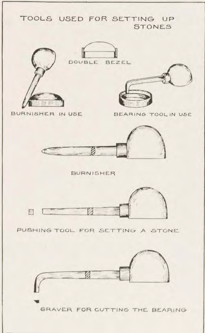
FIG. 44. SETTING A STONE, AND TOOLS USED
