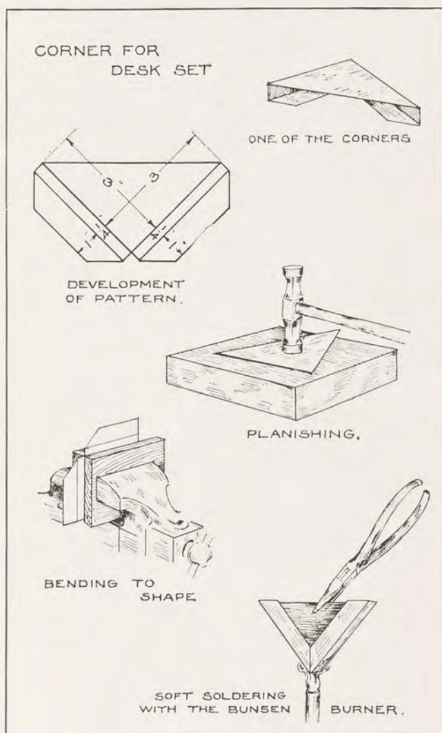
FIG. 129. MAKING THE CORNERS FOR A DESK SET
