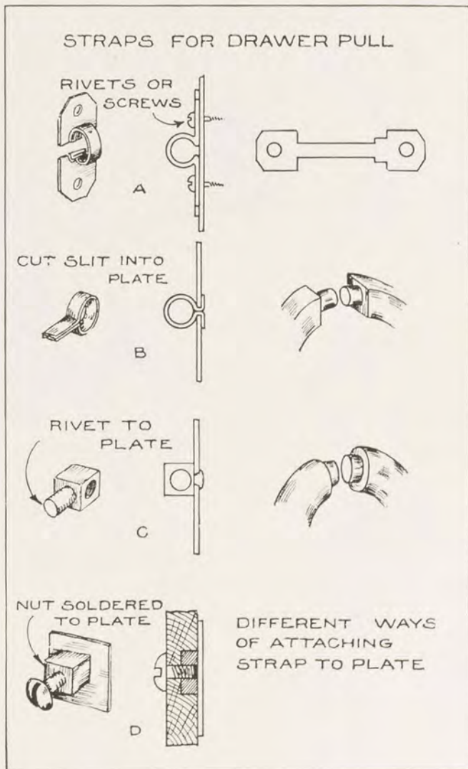
FIG. 115. DIFFERENT METHODS OF FASTENING PULL TO DRAWER PLATE
