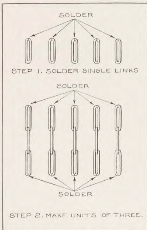
FIG. 94. THE MAKING OF A CHAIN
