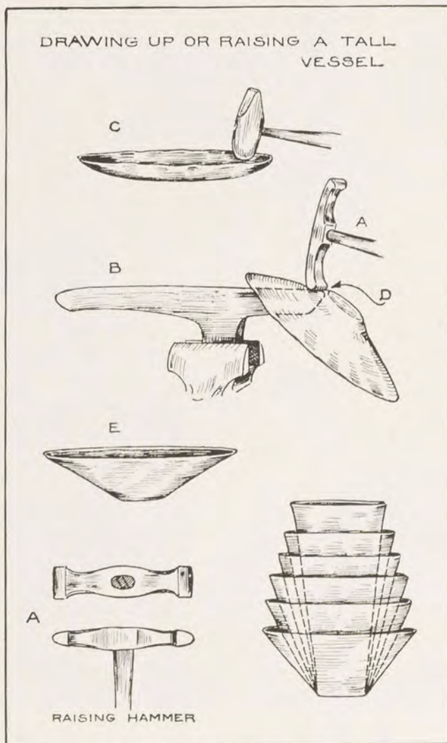
FIG. 138. SUCCESSIVE STEPS IN RAISING A VESSEL FROM A FLAT CIRCULAR SHEET OF METAL
