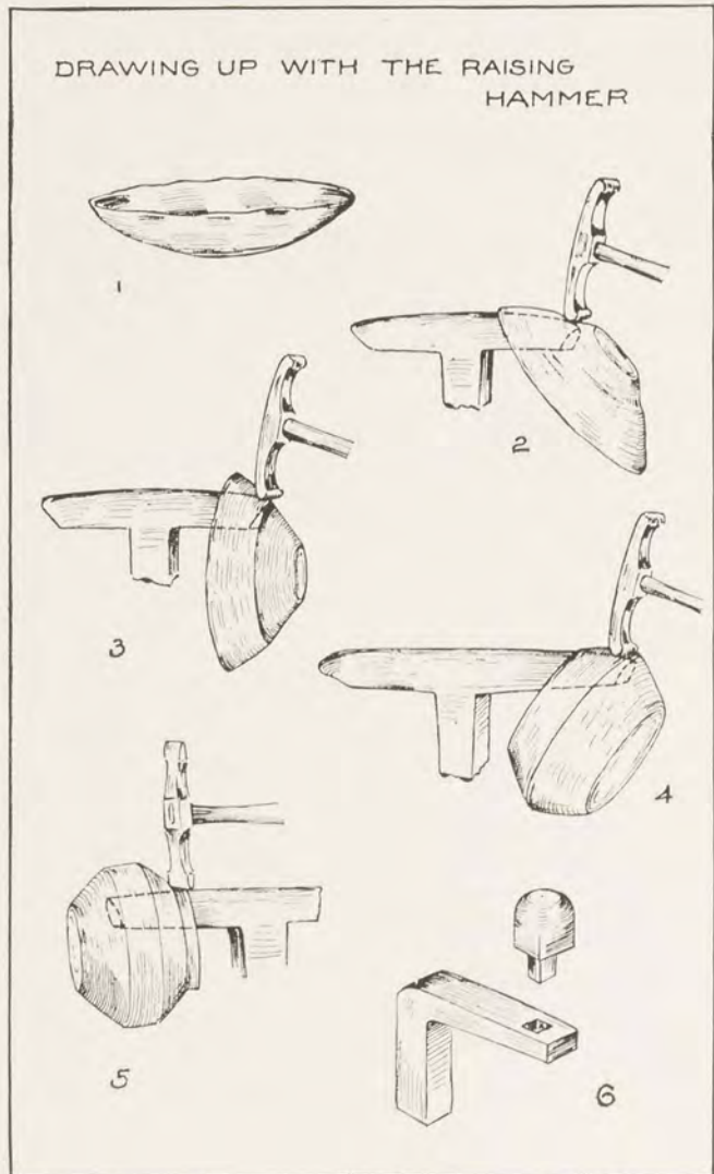
FIG. 140. SUCCESSIVE STEPS IN DRAWING UP A PIECE OF WORK
