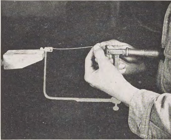
FIG. 14. THE SAW BLADE BEING CLAMPED INTO PLACE
