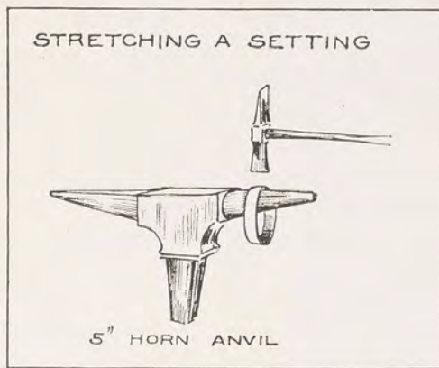
FIG. 35. JEWELER'S HORN ANVIL IN USE
