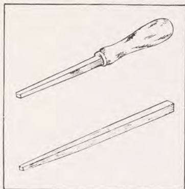
FIG. 43. PUSHING TOOLS USED FOR SETTING A STONE
