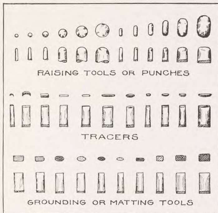
FIG. 70. CHASING TOOLS, THE MOST IMPORTANT SHAPES
