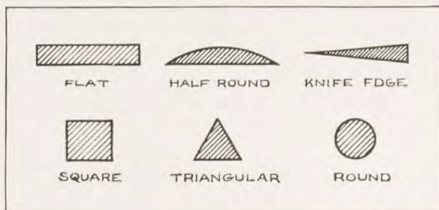
FIG. 16. CROSS-SECTIONS OF FILES
