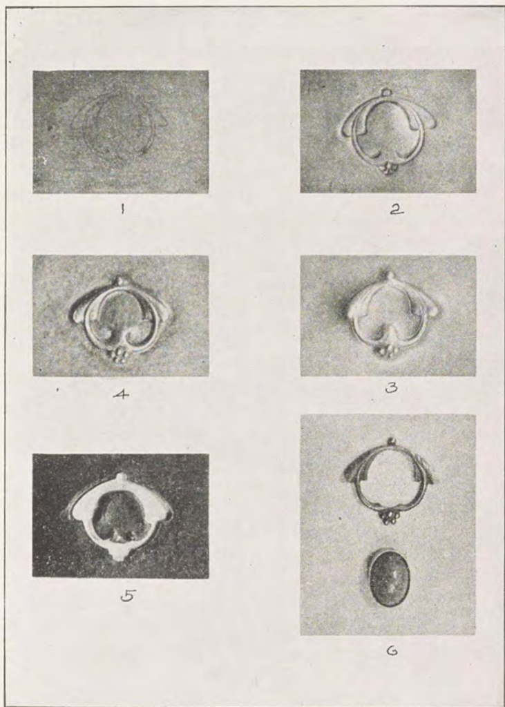
FIG. 68. SHOWING THE DIFFERENT STEPS IN MAKING A SCARF PIN IN REPOUSSÉ WORK
