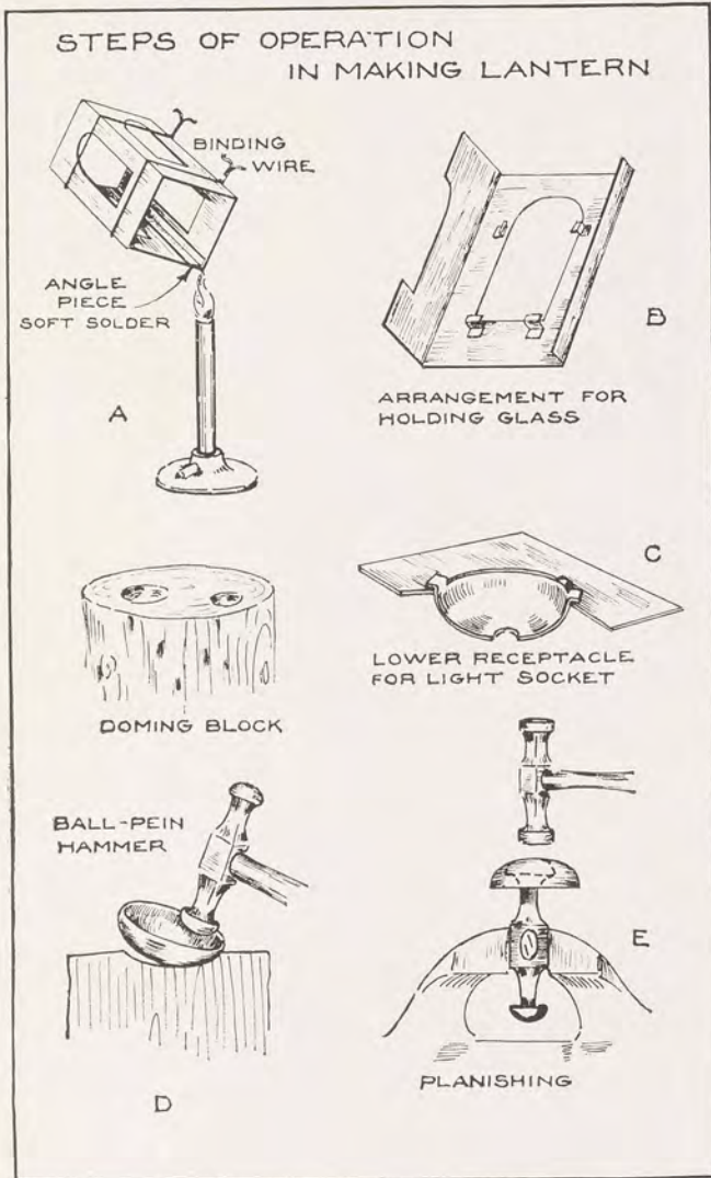
FIG. 122. IMPORTANT STEPS IN MAKING WALL LANTERN
