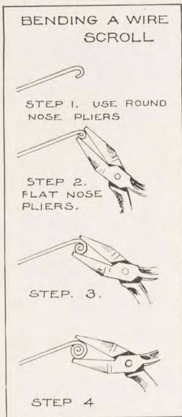
FIG. 98. HOW TO MAKE A WIRE SPIRAL
