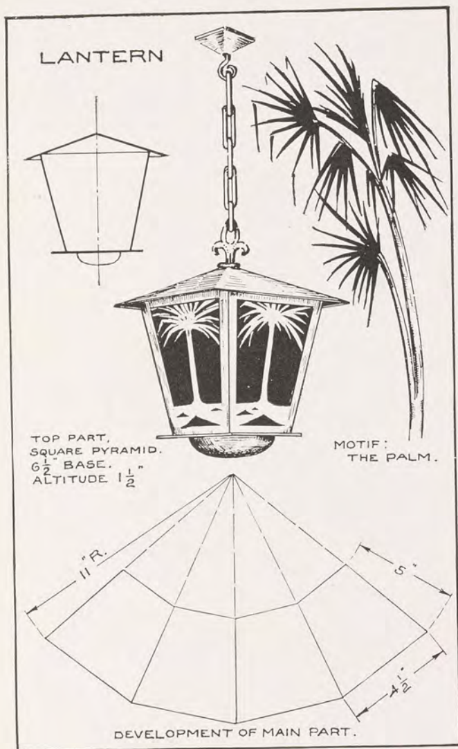
FIG. 124. CEILING LANTERN, INVERTED PYRAMID SHAPE, WITH MOTIF FOR DESIGN
