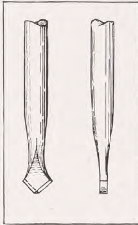
FIG. 12. DRILL POINTS
