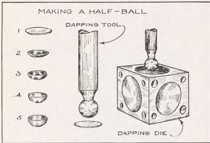
FIG. 120. THE DAPPING DIES AND DAPPING TOOLS
