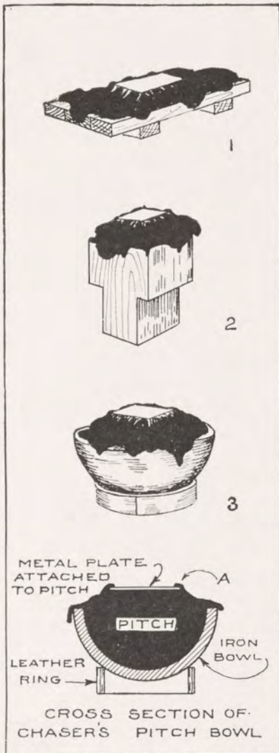
FIG. 69. DIFFERENT WAYS OF ATTACHING METAL PLATE TO PITCH
