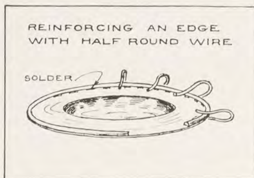
FIG. 147. SOLDERING A WIRE EDGE ON
