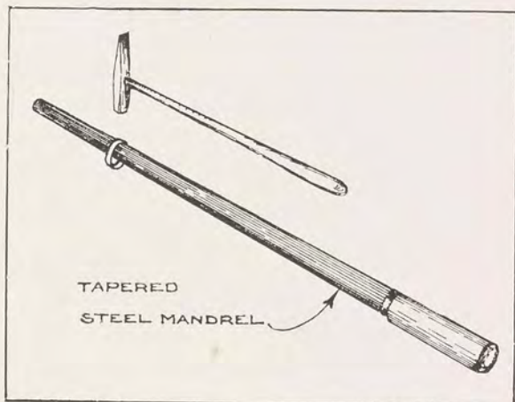
FIG. 34. STRETCHING A BEZEL ON A STEEL MANDREL.
