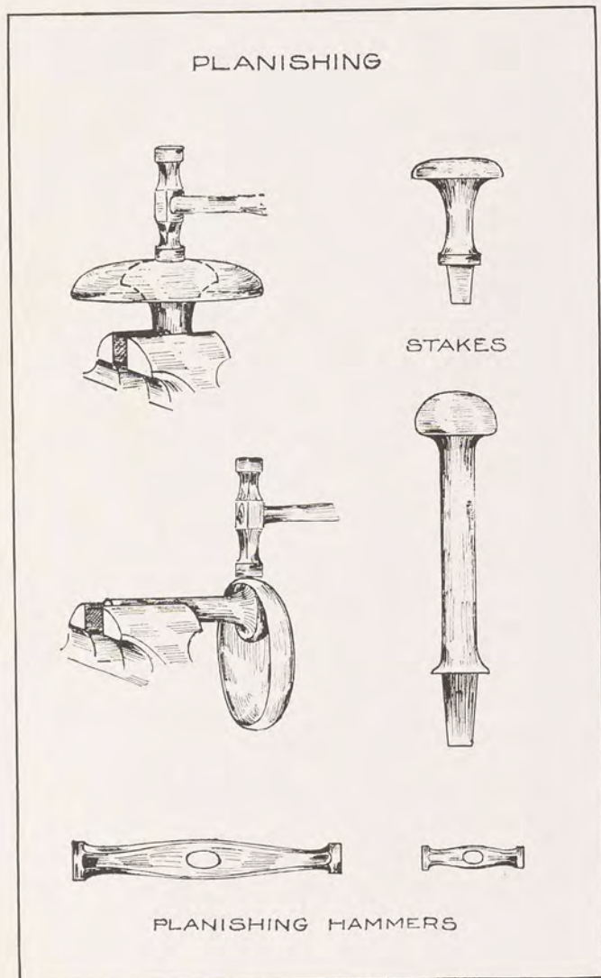
FIG. 135. THE PLANISHING PROCESS
