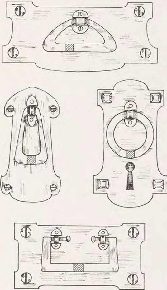
FIG. 114. DESIGNS FOR DRAWER AND DOOR PULLS
