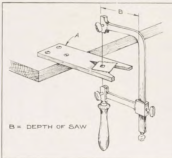
FIG. 13. THE JEWELER'S SAW-FRAME AND CUTTING BOARD
