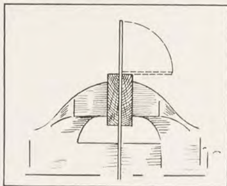
FIG. 111. BENDING A PIECE OF METAL HELD BETWEEN TWO PIECES OF WOOD
