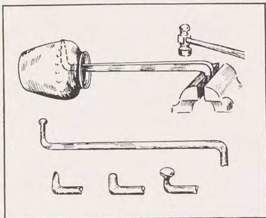
FIG. 86. THE SNARLING IRON IN USE AND VARIOUS SHAPES OF SAME
