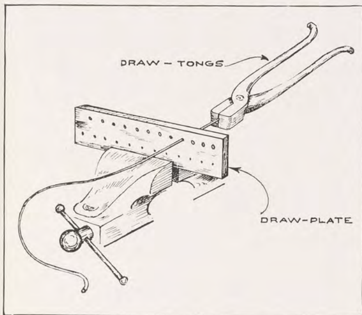
FIG. 17. DRAWING WIRE
