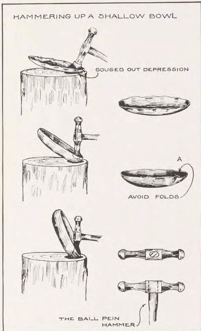
FIG. 133. THE BALL PEIN HAMMER IN USE
