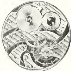
No. 951 Hunting. No. 950 Open Face. Nickel, Bridge Movement, Pendant or Lever Set, 25 Extra Fine Ruby Jewels in Gold Settings, Patent Motor Barrel, Gold Train, Escapement Cap Jeweled, Steel Escape Wheel, Double Roller Escapement, Sapphire Pallets, Breguet Hairspring, Micrometric Regulator, Compensation Balance, Double Sunk Dial, Adjusted to Temperature, Isochronism and Five Positions, $73.50
