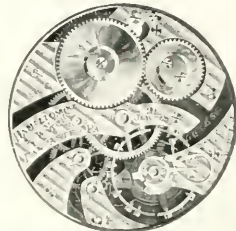
No. 961 Hunting. No. 960 Open Face. Nickel, Bridge Movement, Pendant or Lever Set, 21 Extra Fine Ruby Jewels in Gold Settings, Escapement Cap Jeweled, Steel Escape Wheel, Gold Train, Double Roller Escapement, Sapphire Pallets, Micrometric Regulator, Breguet Hairspring, Compensation Balance, Double Sunk Dial, Adjusted to Temperature, Isochronism and Five Positions, $61.50
