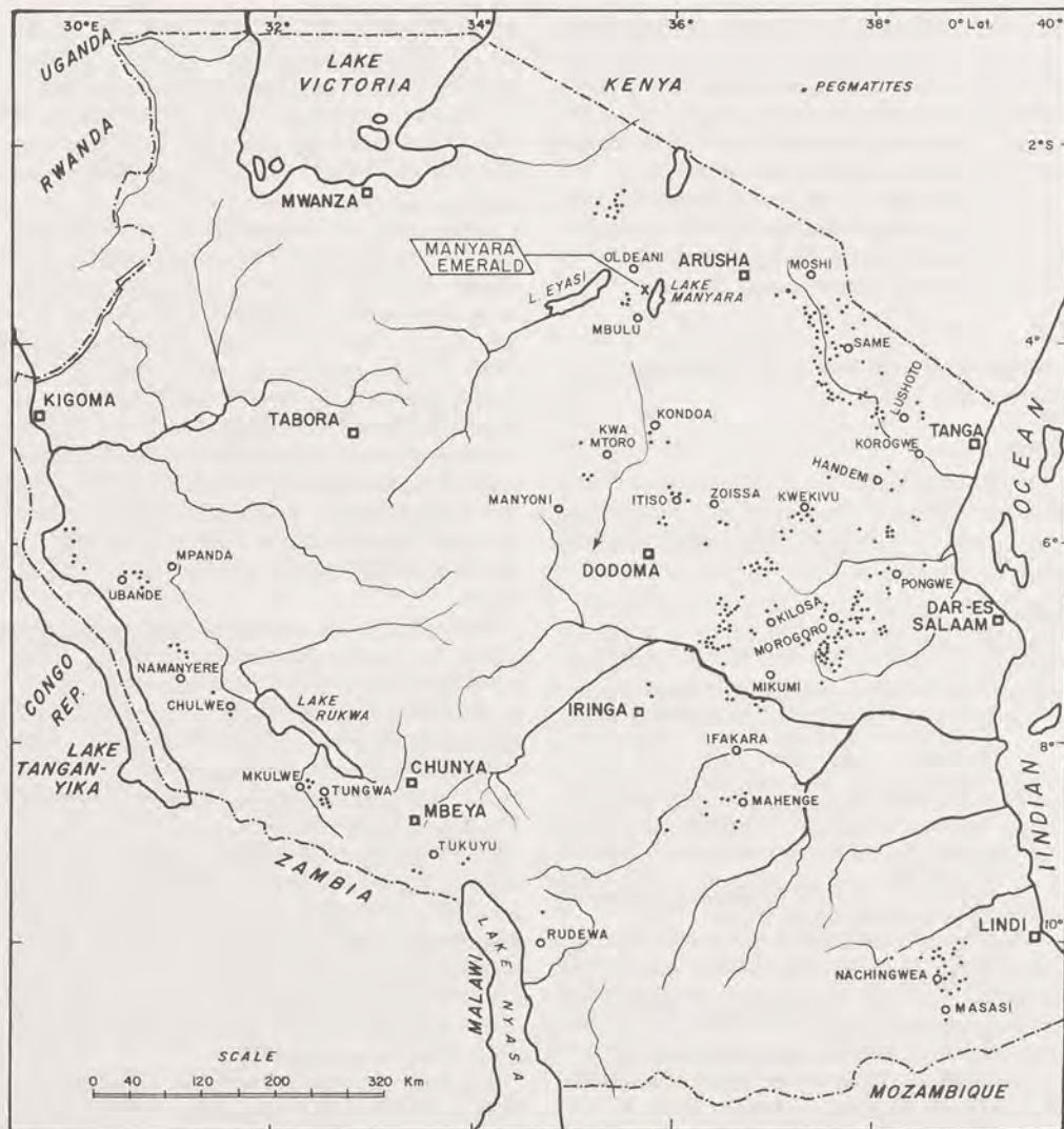
Fig. 14-50 Sketch map of Tanzania showing locations of granitic pegmatites yielding mica and also beryl. The Lake Manyara emerald deposit is also shown. After a map of D. N. Sampson, "The mica pegmatites of Tanzania," Overseas Geology and Mineral Resources 10 (1966).
