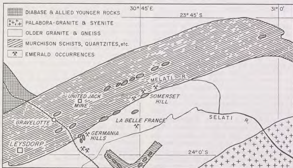
Fig. 14-44 Emerald occurrences in the Leysdorp, Transvaal district, Republic of South Africa. The elongated Murchison series form a folded mass of schists, amphibolites, quartzites, slates, and calcisilicate rocks, among others, resting on granites. The small island structures or "kops" are generally of quartzite. After J. M. Le Grange, "The Barbara Beryls . . ." Transactions of the Geological Society of South Africa 32 (1929).
