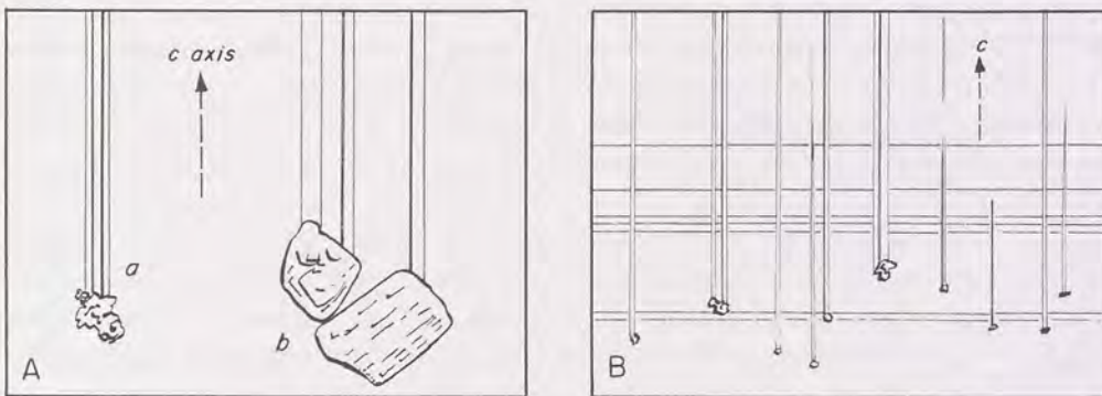
Fig. 10-1 Typical inclusions in beryls. A: Solid inclusions giving rise to face-lined tubes parallel to the c -axis; irregular mass at (a) probably a clay mineral, small crystals at (b), possibly of quartz. B: Similar tubular inclusions passing through color zones, the latter parallel to the basal plane c\{0001\} ; some tubes persist, some are interrupted, and others taper to a closure in the "spike" or "nailhead" inclusions. From V. G. Feklichev, Berill: morfologiya, sostav i struktura kristallov . (Moscow: Izdatelstvo Nauka, 1964) and E. Gübelin, Internal World of Gemstones: Documents from Space and Time (Zurich: ABC Edition, 1973).
