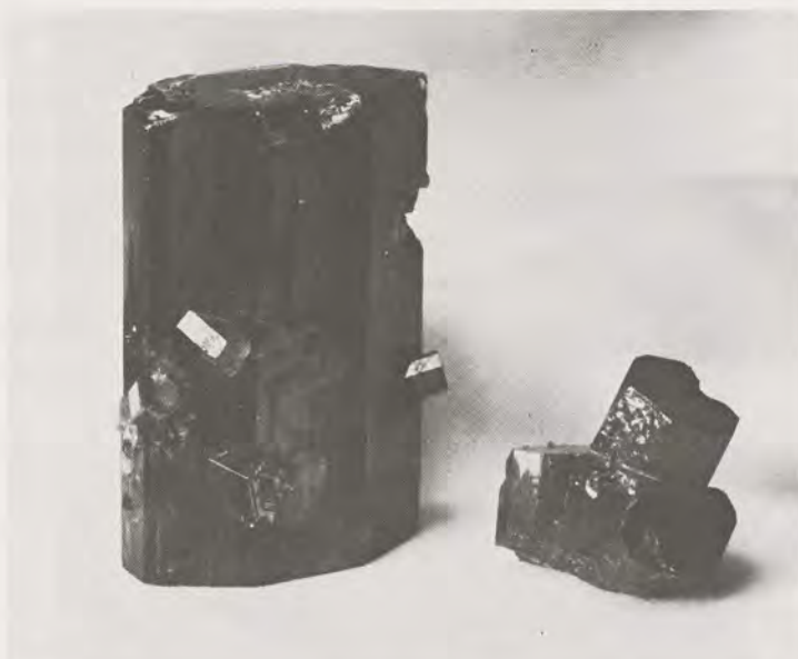
Fig. 11-5 Gilson emerald single crystal and cluster after ten months' growth. The large crystal measures about 63 mm (2½ in) tall and 37 × 12.5 mm (1½ × ½ in) in cross-section; several spontaneously seeded crystals are attached. The cluster crystals show development of second order prisms. Courtesy Labratoire Gilson.
