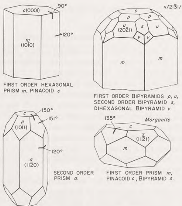
Fig. 9-4 The most common forms found on beryl crystals. The form at the top left is typical of emerald; that at the bottom right is typical of alkali beryls. The two others are common in aquamarines.
