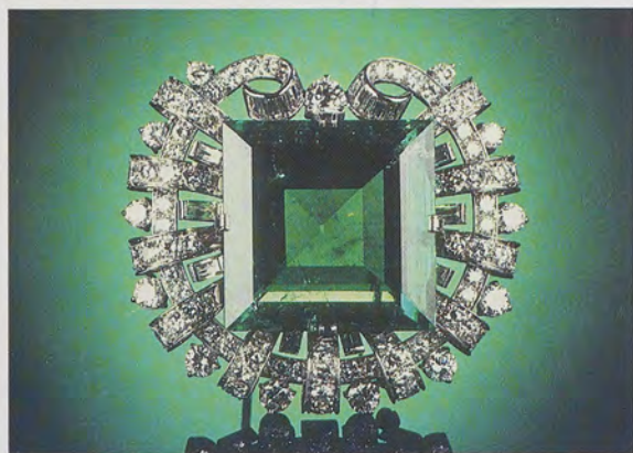
Fig. 20 The Hooker emerald brooch set with a magnificent square-cut emerald of about 75 carats; now in the collections of the National Museum of Natural History, Washington, D.C. Reputedly, the stone once adorned the belt buckle of a Turkish Sultan. Courtesy Smithsonian Institution, Photo No. 77-14194.
