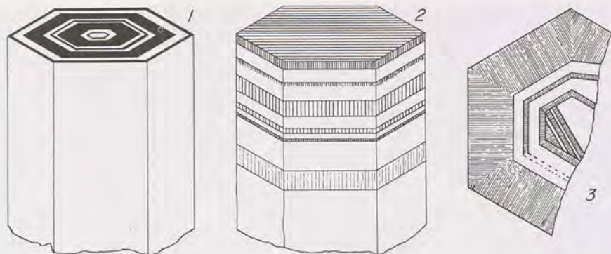
Fig. 8-1 Types of color-zoning in Leysdorp emerald crystals, after J. M. LeGrange, "The Barbara Beryls," Transactions of the Geological Society of South Africa 32 (1929). 1. Zones of colorless or faintly pink alternating with green zones. 2. Less commonly, zones of varying intensity green parallel to the basal pinacoid. 3. Mixed zoning, perhaps due to further growth of emerald upon a fragment of an earlier crystal in which zones were parallel to the c -axis, as in type 1.
