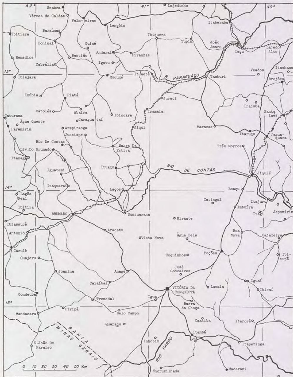
Fig. 14-10 Sketch map of the southeastern portion of the state of Bahia, Brazil showing some beryl localities mentioned in the text.
