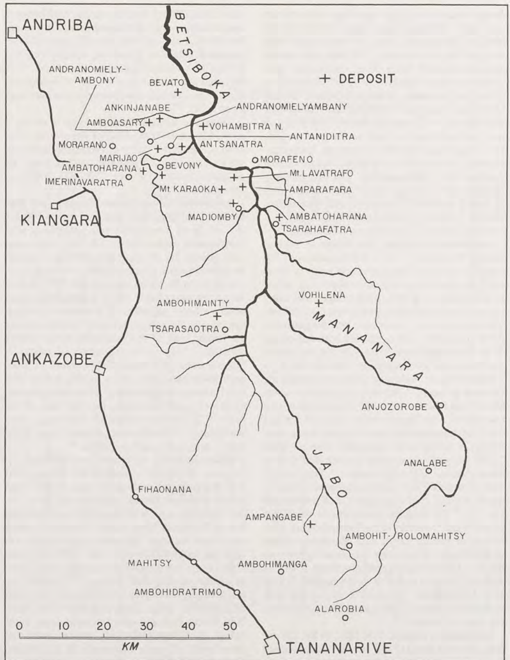
Fig. 14-36 Occurrences of gem beryl in granitic pegmatites in the Ankazobe region northwest of Tananarive. After a map of A. Lacroix, Minéralogie de Madagascar 2 (Paris, 1922).
