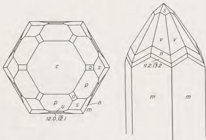
Fig. 14-33 Beryl crystals from Elba showing forms u\{20\bar{2}1\} , v\{213\bar{1}\} , n\{314\bar{1}\} , and the very steep dihexagonal bipyramid \{11.2.13.2\} .
