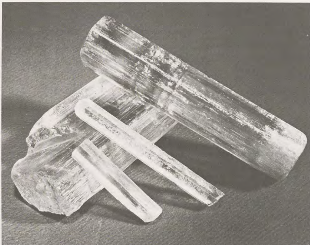
Fig. 8-2 Aquamarine crystals. Top: Terminated, slightly worn simple hexagonal prism with narrow bands of color parallel to the basal plane, from the Nerchinsk region, Transbaikalia, USSR; about 11.5 cm (4½ in) long. The other crystals are from Minas Gerais, Brazil.
