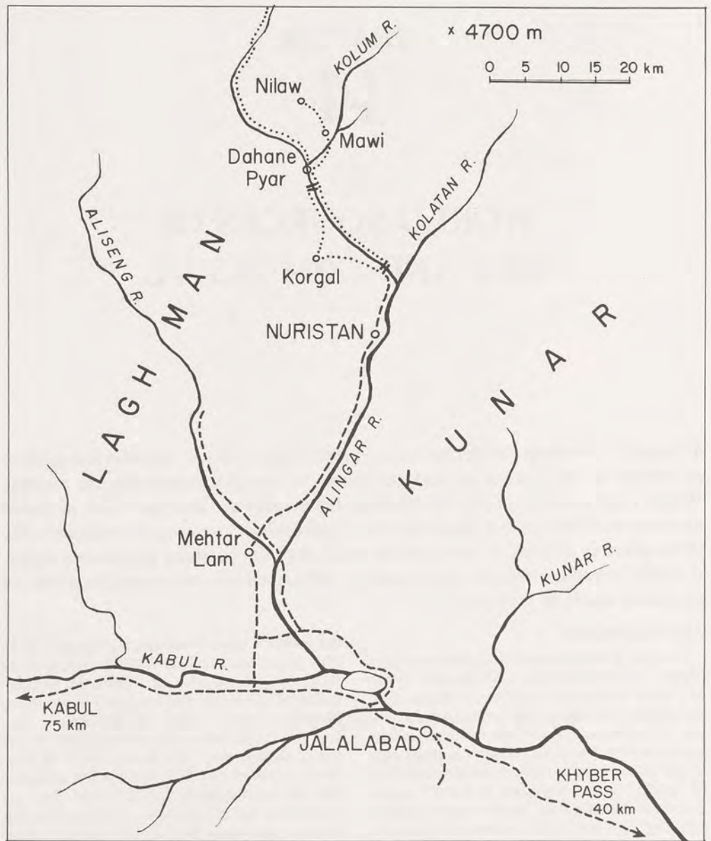
Fig. 14-1 Map of the Nuristan pegmatite region of northeastern Afghanistan. After P. Bariand and J. F. Poullen, "The pegmatites of Laghman, Nuristan, Afghanistan," The Mineralogical Record 9 (1978):303.
