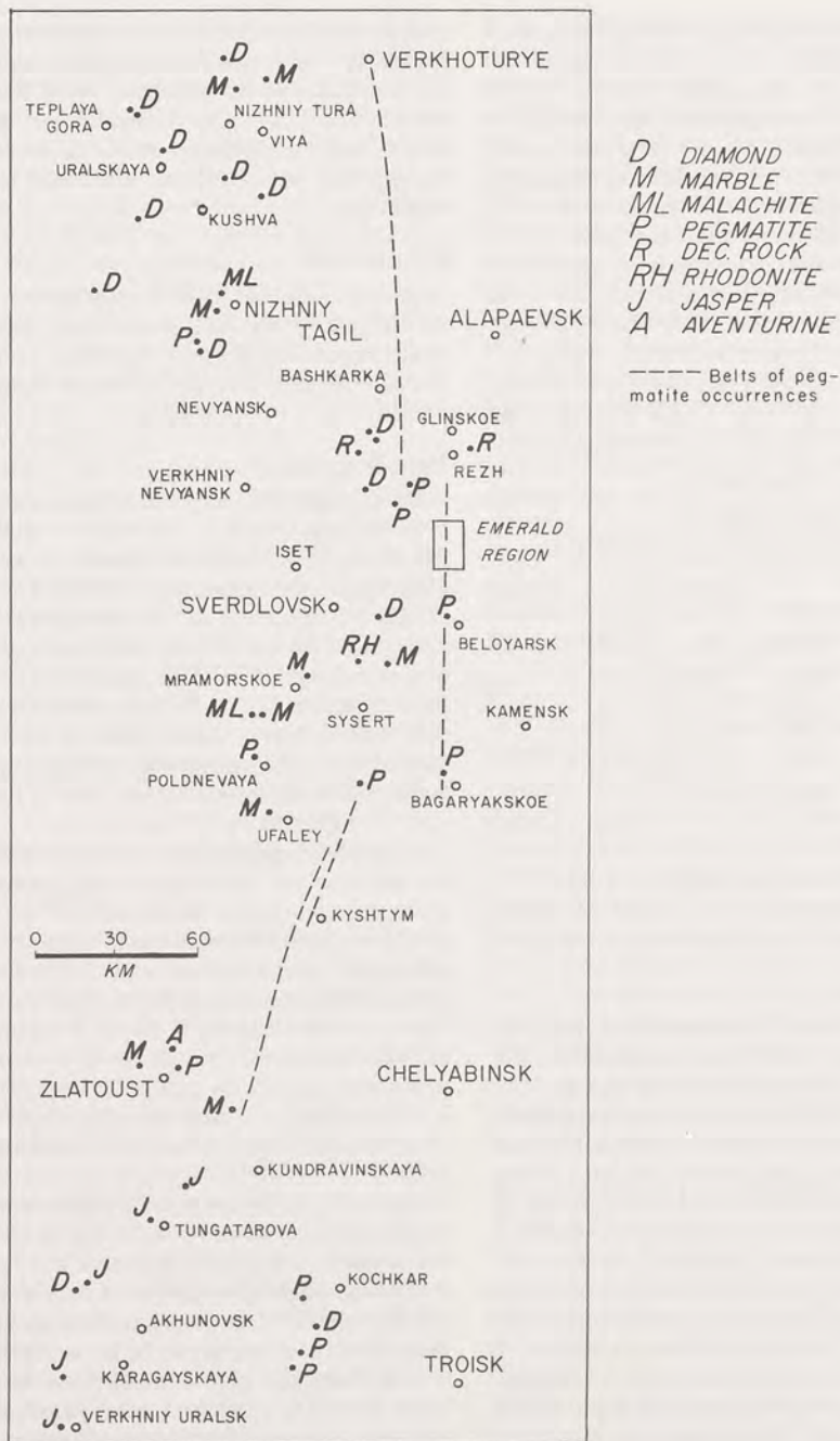
Fig. 14-53 Gemstone deposits along the east flanks of the Ural Mountains, USSR. After the map of A. E. Fersman, Dragotsennyye i Tsvetnyye Kamni , SSSR 2 (Leningrad, 1925).
