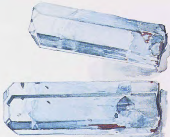
Fig. 8 Two exceptional, transparent terminated aquamarine crystals from the famous Kleine Spitzkopje locality in South West Africa; largest crystal is 54 x 19 mm (2.2 x 0.75 in). William Larson Collection, Fallbrook, California.
