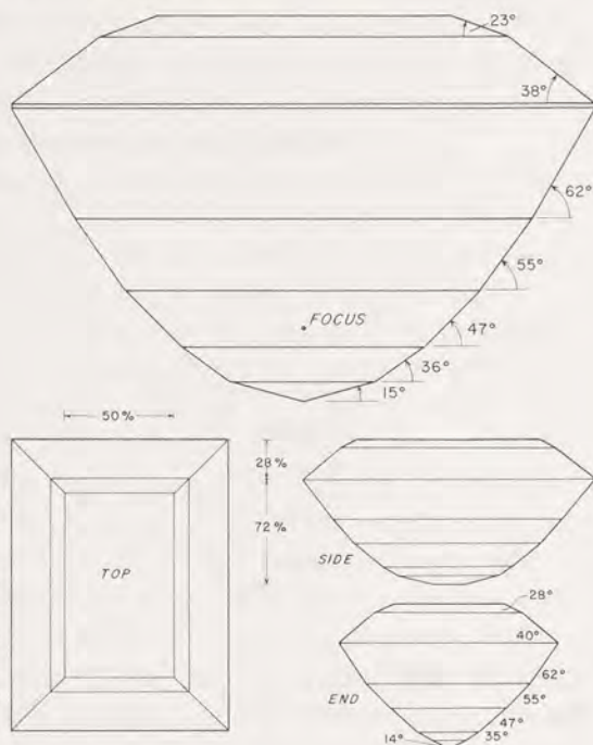
Fig. 12-2 Angles and proportions of cut emeralds advocated by A. M. Barriga Villalba and A. M. Barriga del Diestro in La Esmeralda de Colombia (Bogota: Colegio Mayor de Nuestra Señora del Rosario, 1973). The pavilion facets closely approximate the curvature of a parabola, the focus of which is shown in the top figure. Slightly different angles are shown in a similar cut below.
