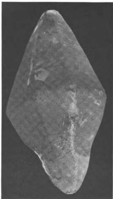
HUGE CRYSTAL OF YELLOW SAPPHIRE (ACTUAL SIZE).
