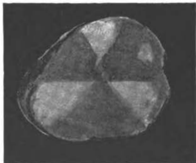
SECTION OF PARTI-COLOURED AMETHYST.
