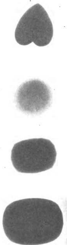
RADIOGRAPH OF FOUR GEMS: OPAL, BRILLIANT, BERYL, SAPPHIRE.
