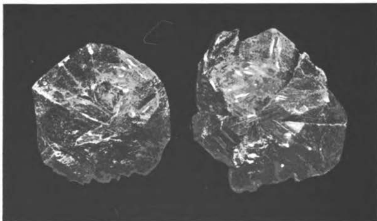
CRYSTALS OF ALEXANDRITE (ACTUAL SIZE).
