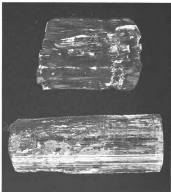
CRYSTALS OF BERYL (ACTUAL SIZE).
