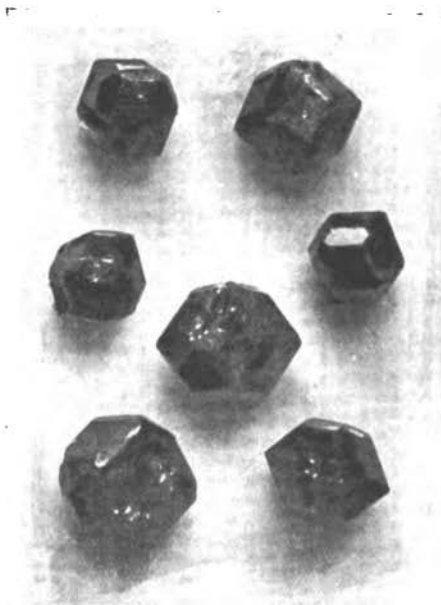
CRYSTALS OF GARNET (ACTUAL SIZE).
