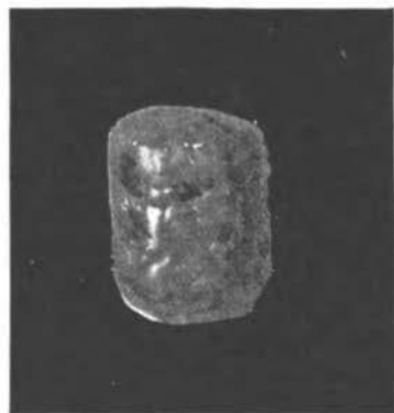
WATER-WORN CRYSTAL OF RUBY (ACTUAL SIZE).
