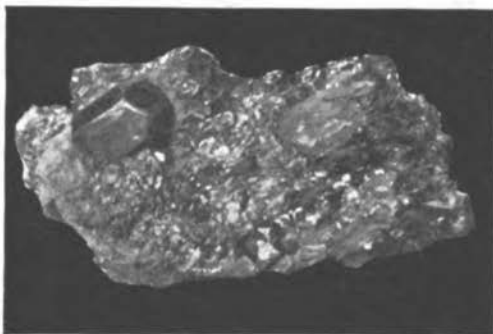
CRYSTAL OF ZIRCON OR JARGOON IN MATRIX.
