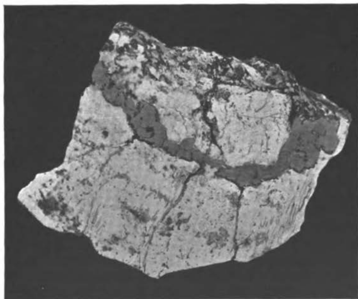
TURQUOISE IN THE FORM OF A VEIN.
