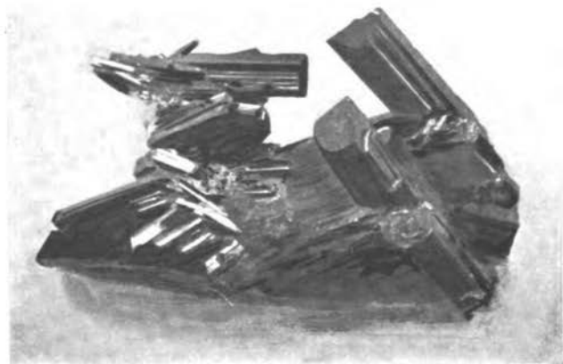
CRYSTALS OF EPIDOTE (ACTUAL SIZE).
