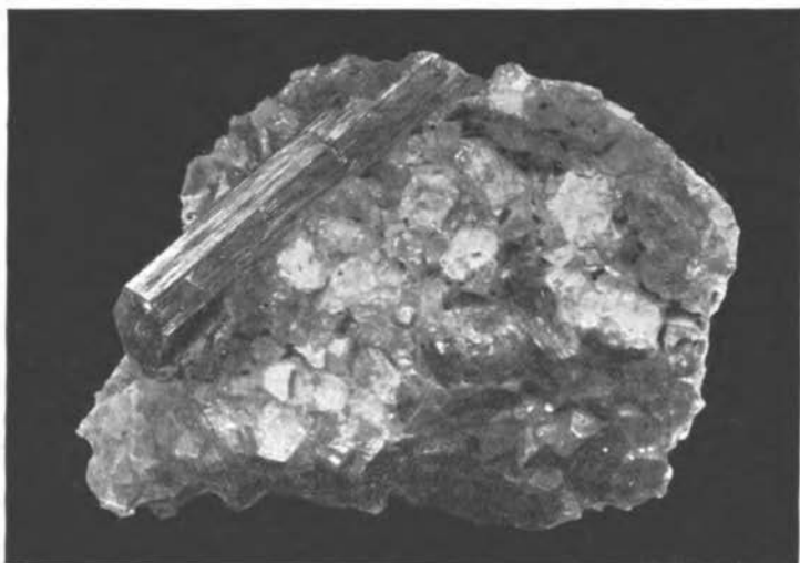
CRYSTAL OF BERYL ON TOPAZ.
