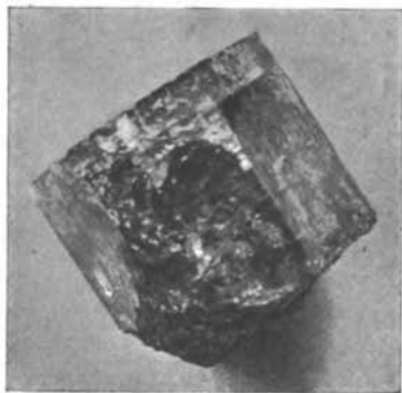
LARGE ROUGH EMERALD (FRAGMENTARY).
