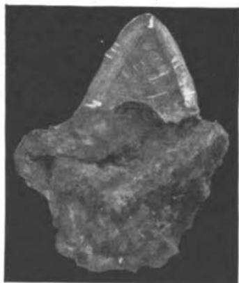
CRYSTAL OF SPHENE IN MATRIX (ACTUAL SIZE).
