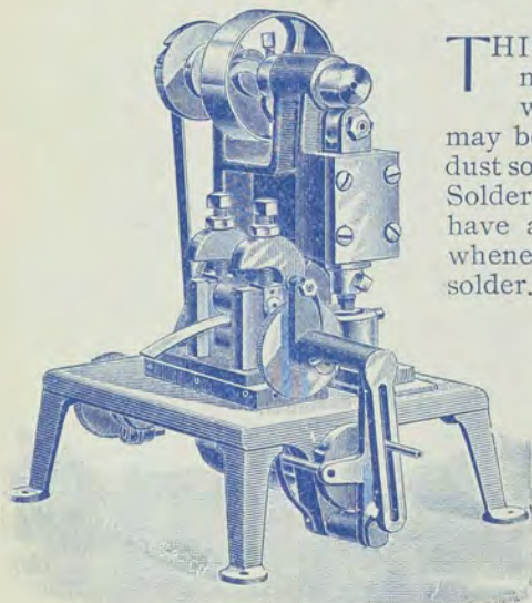
AUTOMATIC SOLDER CUTTER.
