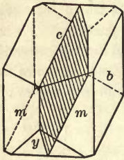
Fig. 3. Symmetry Plane.
