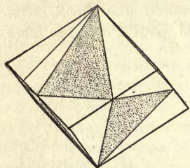
Fig. 119. Showing Relation between First Order Pyramid and Rhombohedron.
