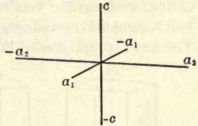
Fig. 76. Tetragonal Axes.
