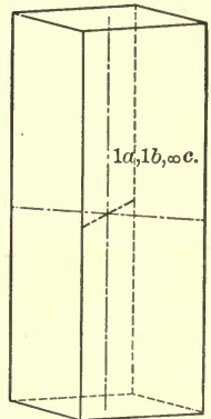
Fig. 8. Orthorhombic Prism.
