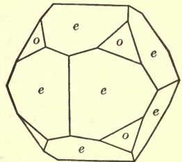
Fig. 59. Pyritohedron and Octahedron.
