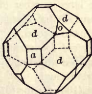
Fig. 74. Dodecahedron, Cube and Tetrahedron.
