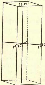
Fig. 144. Axes of Symmetry. Orthorhombic System.
