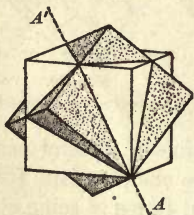
Fig. 21. Twinned Cubes.
