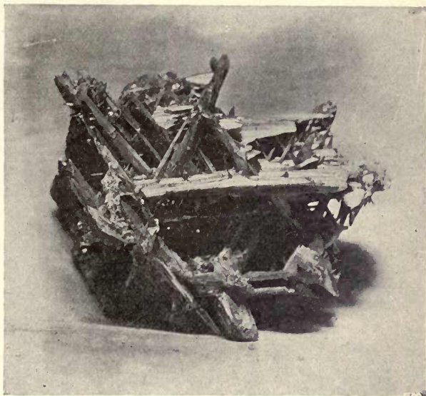
Cerussite, Broken Hill, New South Wales.
