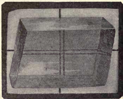
Fig. 196. Double Refraction in Calcite.
