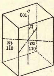
Fig. 169. Prism and Base.
