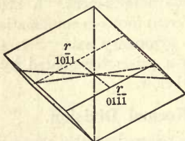
Fig. 120. Positive Rhombohedron.
