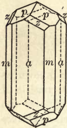
Fig. 100. Scapolite.
