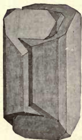
Fig. 291. Carlsbad Twin.
