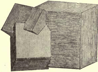
Fig. 226. Striated Cubes.
