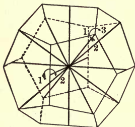
Fig. 50. Symmetry of Pyritohedral Class, Isometric System.
