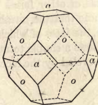
Fig. 32. Octahedron and Cube.
