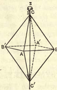
Fig. 4. Symmetry Axis.
