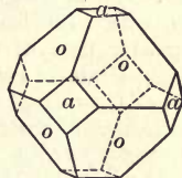
Fig. 219. Octahedron and Cube.
