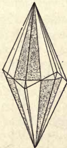
Fig. 131. Showing Relation between Dihexagonal Pyramid and Scalenohedron.
