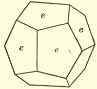
Fig. 227. Pyritohedron
