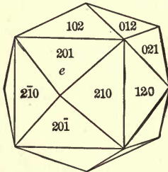
Fig. 38. Tetrahexahedron.
