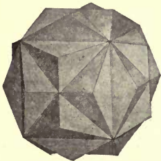
Fig. 231. Twinned Pyritohedrons.
