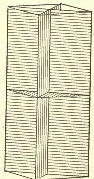
Fig. 145. Planes of Symmetry. Orthorhombic System.
