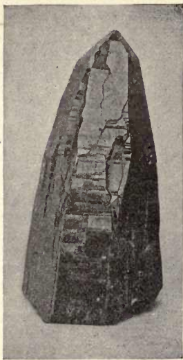
A. Smoky Quartz, Pike's Peak, Colorado.
