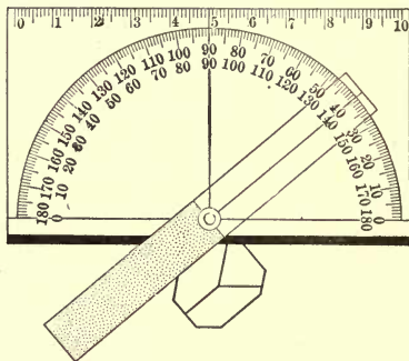
Fig. 2. Contact Goniometer.
