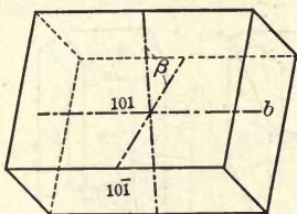
Fig. 170. Orthodomes and Clinopinacoid.
