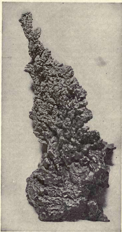
Arborescent Copper, Lake Superior.
