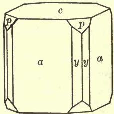
Fig. 94. Apophyllite.
