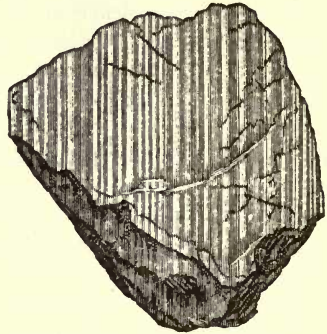
Fig. 298. Albite Twinning.
