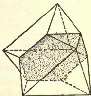
Fig. 22. Twinned Octahedron.
