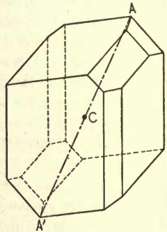
Fig. 5. Symmetry Center.
