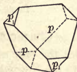
Fig. 99. Positive and Negative Sphenoids.
