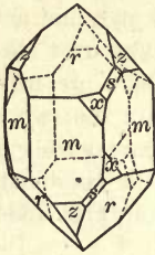
Fig. 141. Right-handed Quartz.
