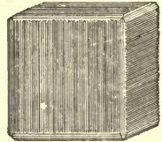
Fig. 55. Striated Cube.
