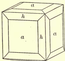
Fig. 213. Cube and Tetrahexahedron.
