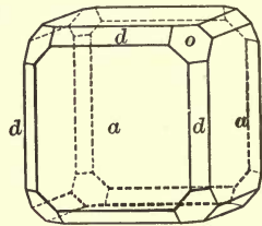
Fig. 37. Cube, Octahedron and Dodecahedron.
