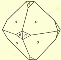
Fig. 57. Octahedron and Pyritohedron.
