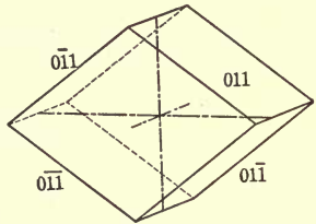
Fig. 149. Brachydome and Macropinacoid.
