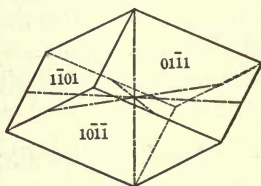
Fig. 121. Negative Rhombohedron.
