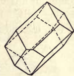
Fig. 20. Distorted Dodecahedron.
