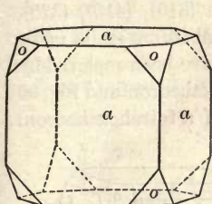
Fig. 31. Cube and Octahedron.
