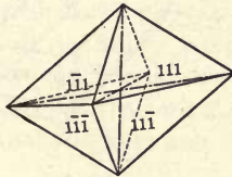
Fig. 181. Pyramids.
