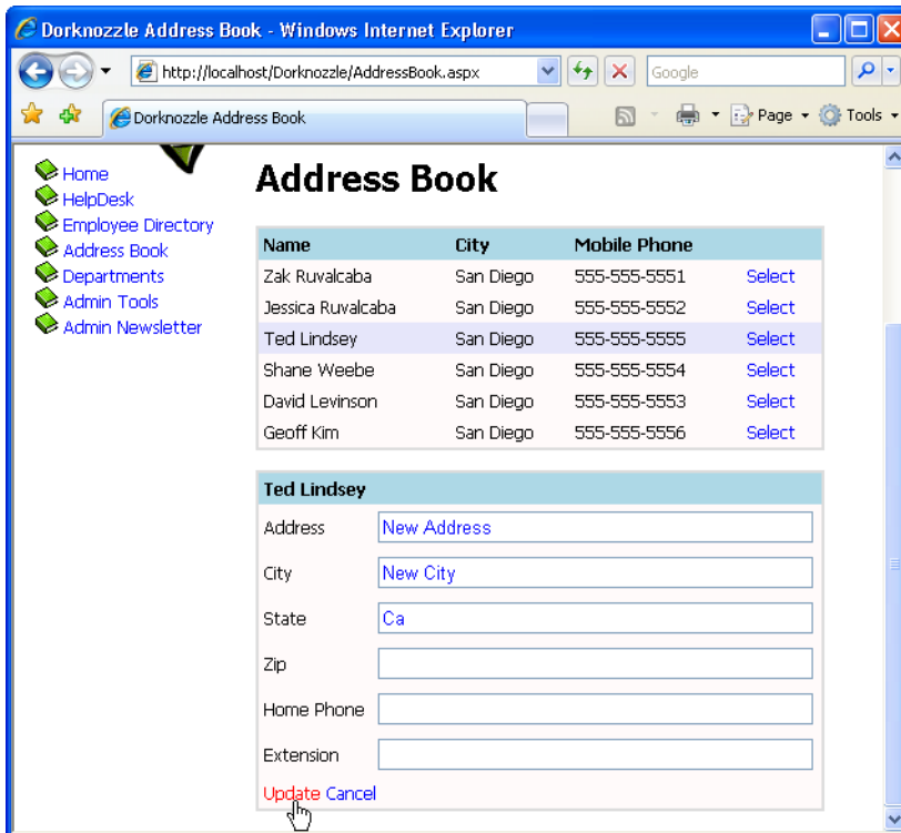
Figure 11.18. Updating an employee's address and city
