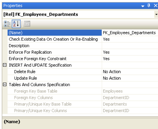
Figure 7.28. The properties of a foreign key
