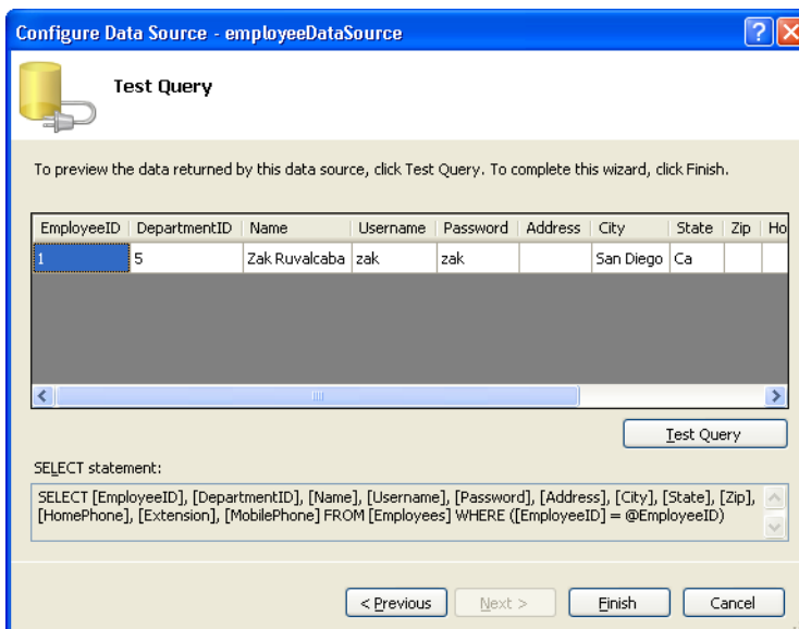
Figure 12.12. Testing the query generated for our data source
