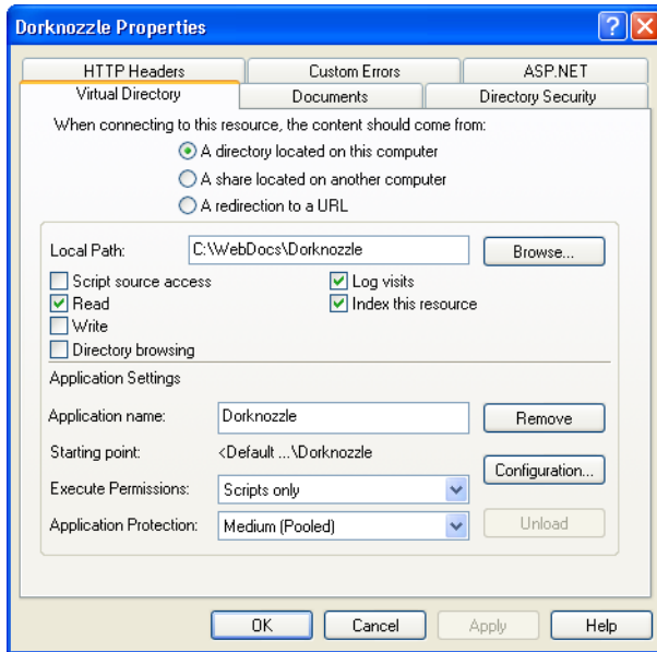
Figure 5.21. Editing the virtual directory's properties
