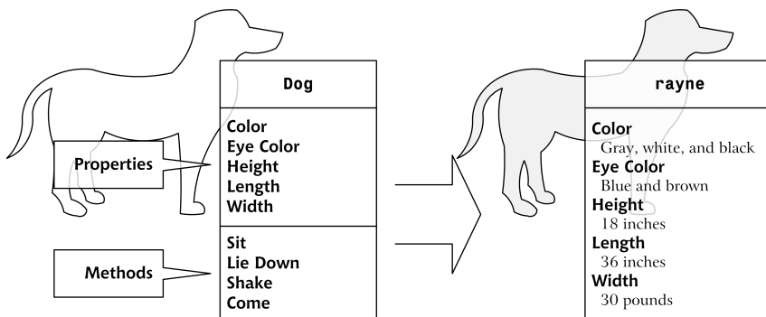
Figure 3.6. An instance of Dog
