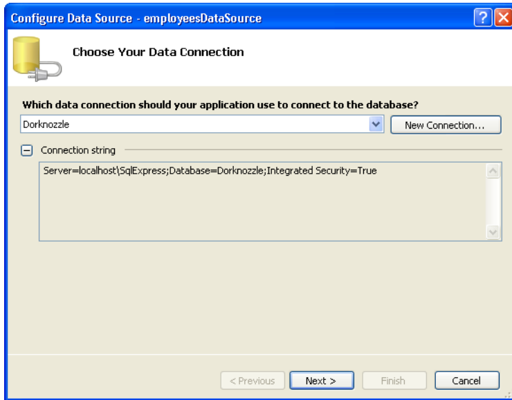
Figure 12.3. Specifying the connection string
