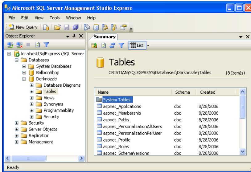
Figure 13.9. Membership tables in Dorknozzle
