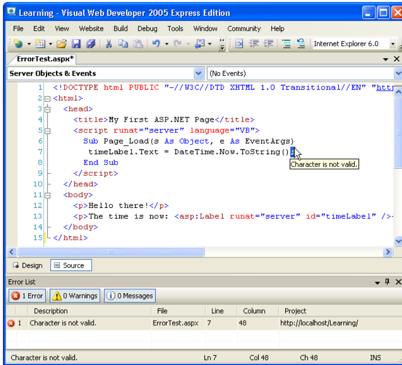
Figure 5.55. Visual Web Developer explaining an error in a tooltip
