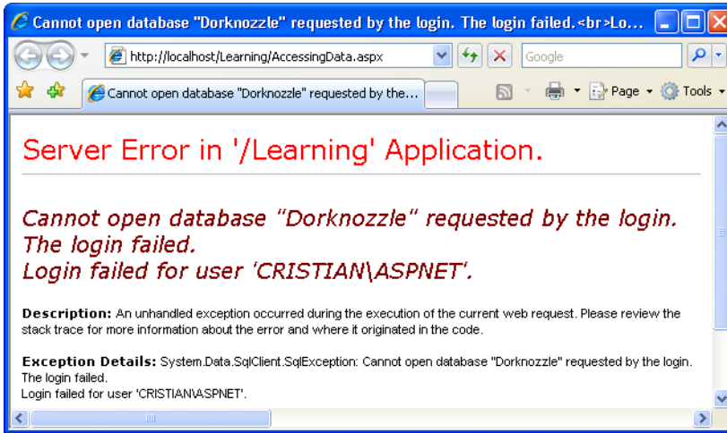
Figure 9.2. A database connection error trapped by the ASP.NET runtime
