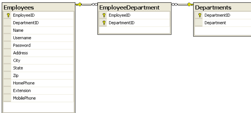
Figure 7.29. Using a mapping table to implement a many-to-many relationship
