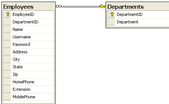
Figure 7.27. Database diagram showing a one-to-many relationship
