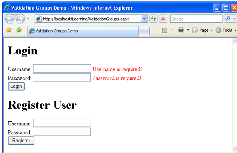
Figure 6.10. Triggering the Login ValidationGroup
