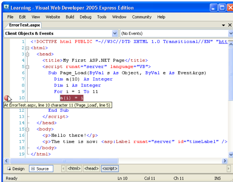
Figure 5.51. Setting a breakpoint
