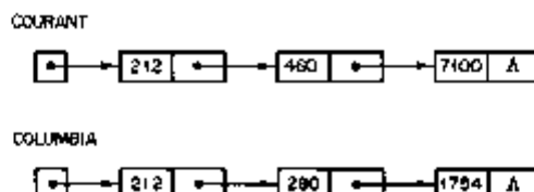
Figure 2.2. Two singly linked lists.
