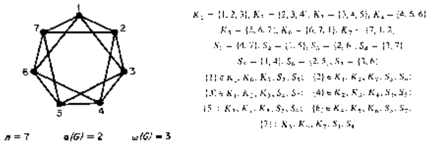
Figure 3.2. The graph \bar{G} , and its maximum clique and stable set structure as specified in Theorem 3.1E.
