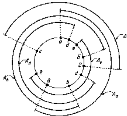
Figure 8.11. A collection of arcs of a circle with representing sequence of endpoints \sigma = [a, \bar{a}, c, \bar{c}, \bar{b}, \bar{d}, \bar{d}, b, \bar{a}, \bar{e}, c]
