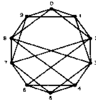
Figure 3.5. A graph satisfying the Lovász and Padberg conditions which fails to be p -critical. The clique matrix and stable set matrix indicate the required indexing of the maximum cliques and maximum stable sets. This example was discovered independently by Huang [1976] and by Chvátal, Graham, Perold, and Whitesides [1979].
