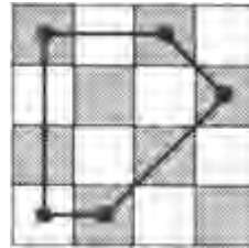
Figure 9.12. A chordless 5-cycle in (F_4, Q) .
