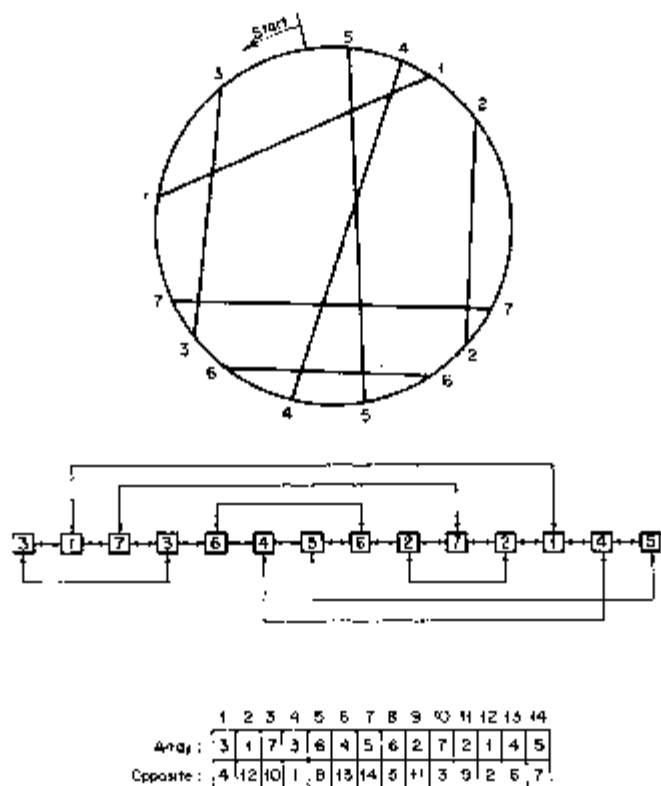
Figure 11.6. Data structures for a circle with chords.
