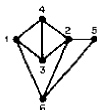
Figure 7.1. The graph G[4, 3, 6, 1, 5, 2] .
