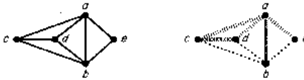
Figure 5.2. An undirected graph G and a coloring of its edges according to the classes of \mathcal{S}(G) .
