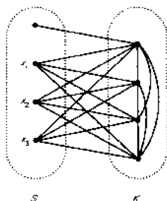
Figure 6.1. A split graph with one of its four partitions indicated. The other partitions are \{S - \{x_i\} \cup (K \cup \{x_i\}) for i = 1, 2, 3 .
