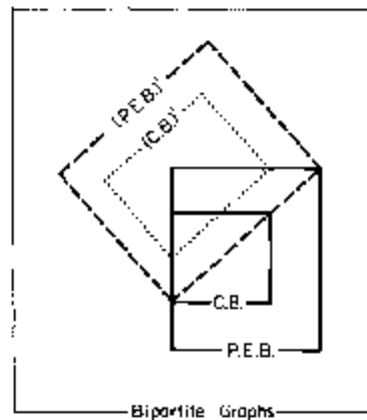
Figure 12.10. Bipartite graphs.
