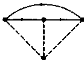
Figure 8.9. Solid edges are in the transitive orientation F of \bar{G} = (V, E) . Broken edges are in G = (V, E) .
