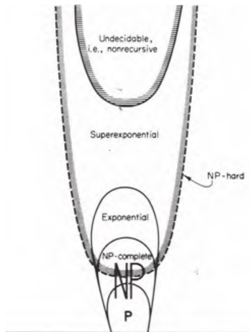
Figure 2.1. The hierarchy of complexities. The big open question is whether or not the "zone of uncertainty," \text{NP} \setminus \text{P} , is empty.
