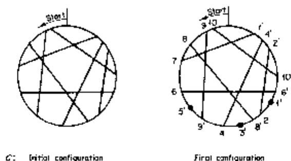
Figure 11.5. Algorithm 11.2 applied to the circle \mathcal{S} . The instructions executed are the following.
