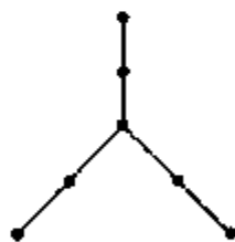
Figure 9.6. \bar{G} : superperfect.
