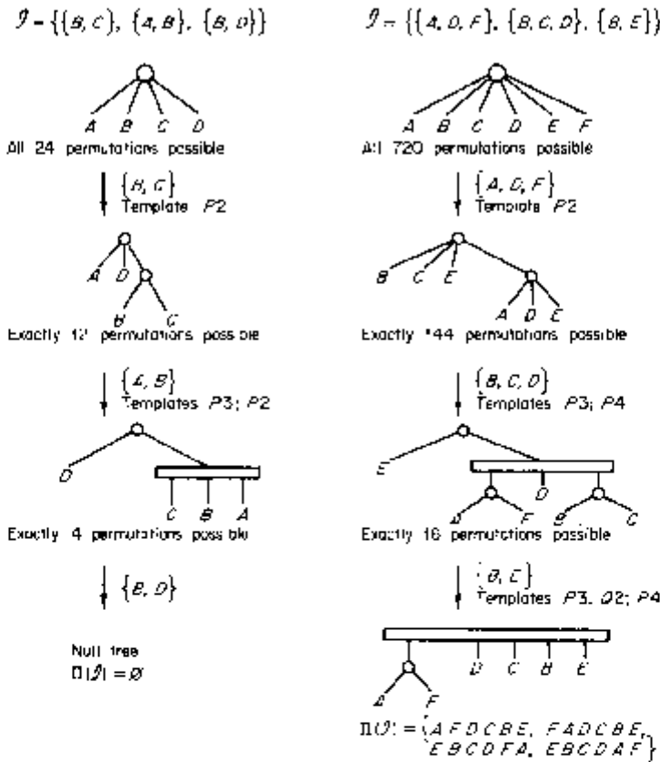
Figure 8.7. Two illustrations of the procedure CONSECUTIVE (PQ-tree version). The reductions make use of the templates in Booth and Leucker [1976]
