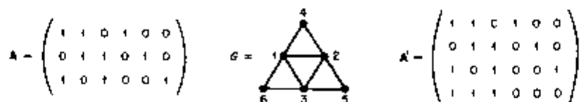
Figure 3.4. The derived graph G of the matrix A is a perfect graph, yet P(A) has (\frac{1}{2}, \frac{1}{2}, \frac{1}{2}, 0, 0, 0) as an extremum; thus A is an imperfect matrix. A' is the clique matrix of G and is perfect.
