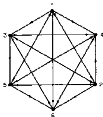
Figure 2.8. A transitive tournament.
