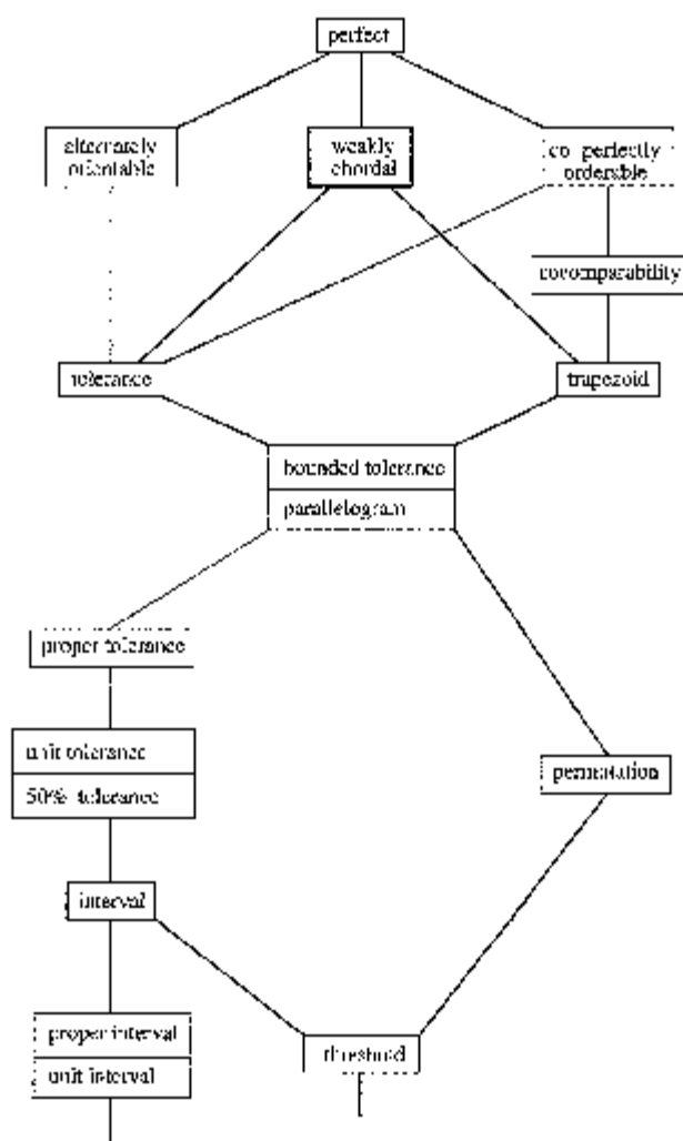
Fig.13.3. A complete hierarchy of classes of perfect graphs ordered by inclusion. Reprinted from Golombic and Trenk [2004].
