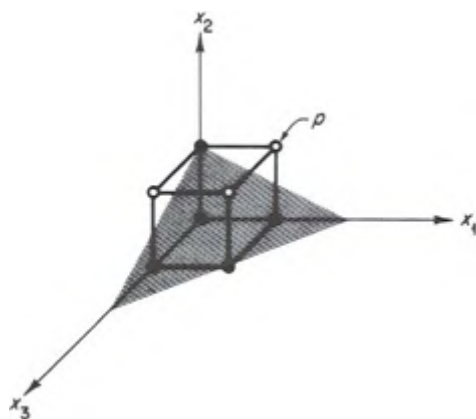
Figure 10.2. The point p = (1, 1, 0) corresponds to the set \{v_1, v_2\} , which is not stable.
