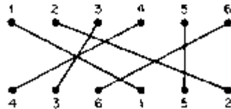
Figure 7.5. The matching diagram of [4, 3, 6, 1, 5, 2] .
