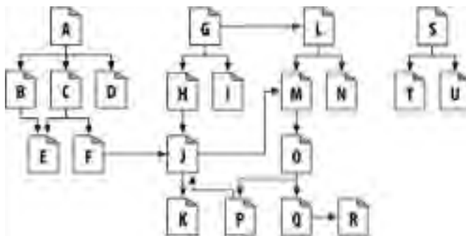
Figure 9-1. A root set is needed to reach all pages
