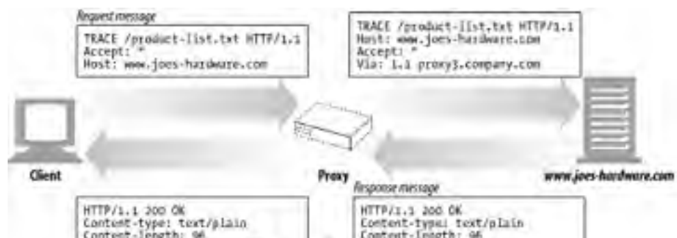
Figure 3-11. TRACE example
