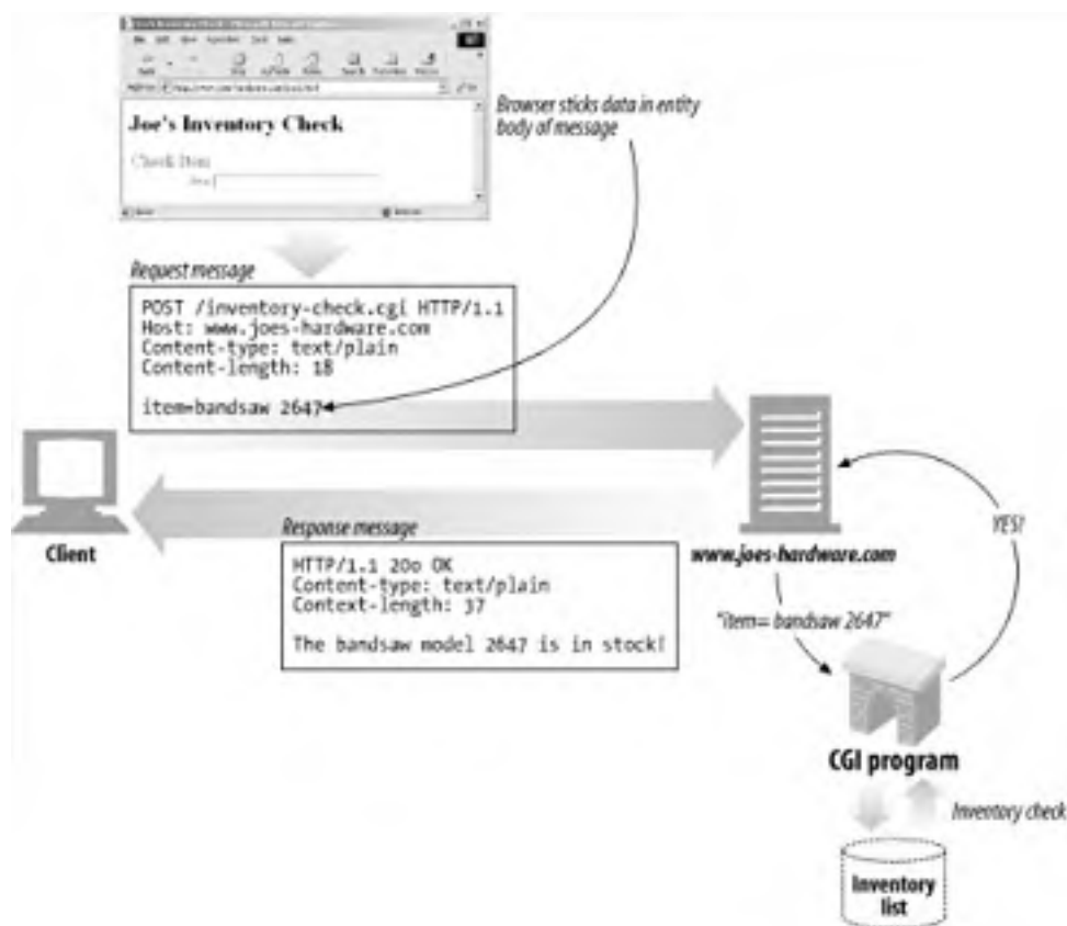
Figure 3-10. POST example
