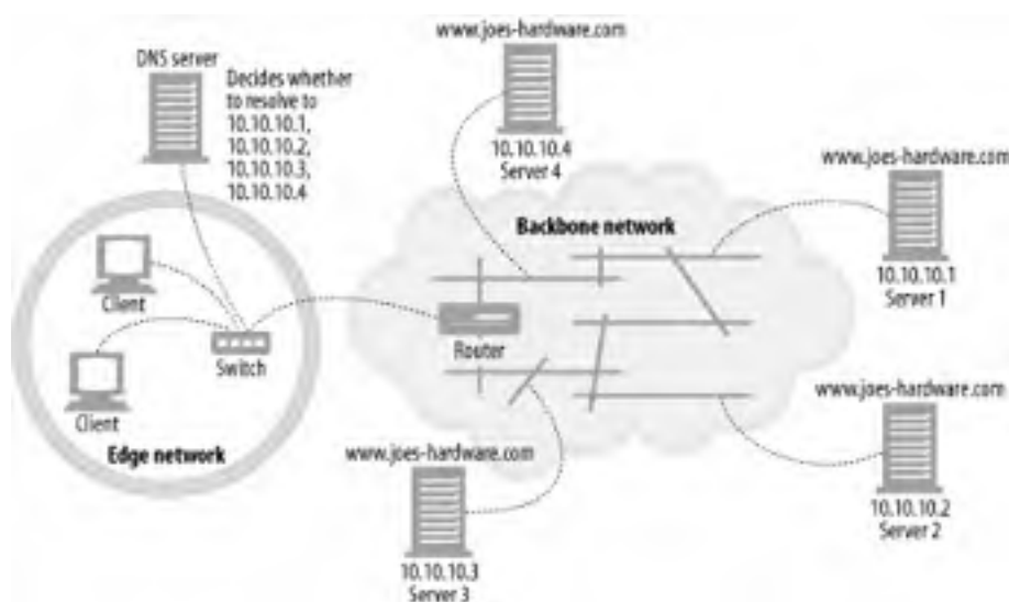
Figure 20-2. DNS-based redirection
