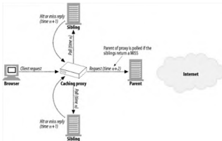
Figure 20-13. ICP queries
