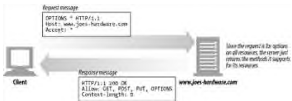
Figure 3-12. OPTIONS example
