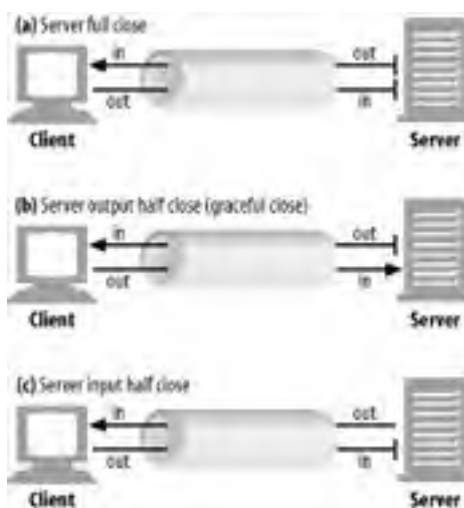
Figure 4-20. Full and half close
