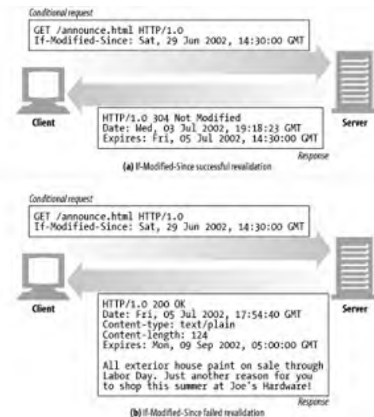
Figure 7-14. If-Modified-Since revalidations return 304 if unchanged or 200 with new body if changed
