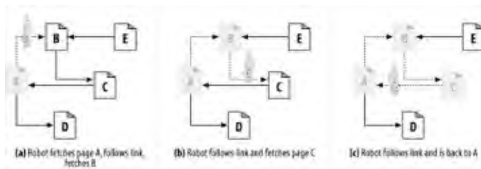
Figure 9-2. Crawling over a web of hyperlinks
