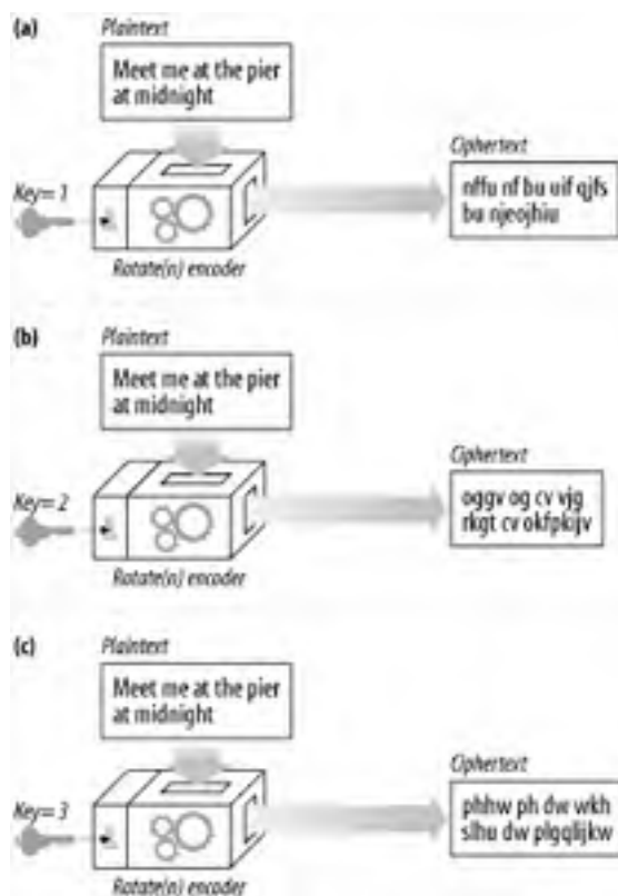
Figure 14-5. The rotate-by-N cipher, using different keys
