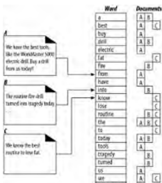
Figure 9-8. Three documents and a full-text index
