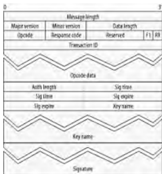
Figure 20-15. HTCP message format
