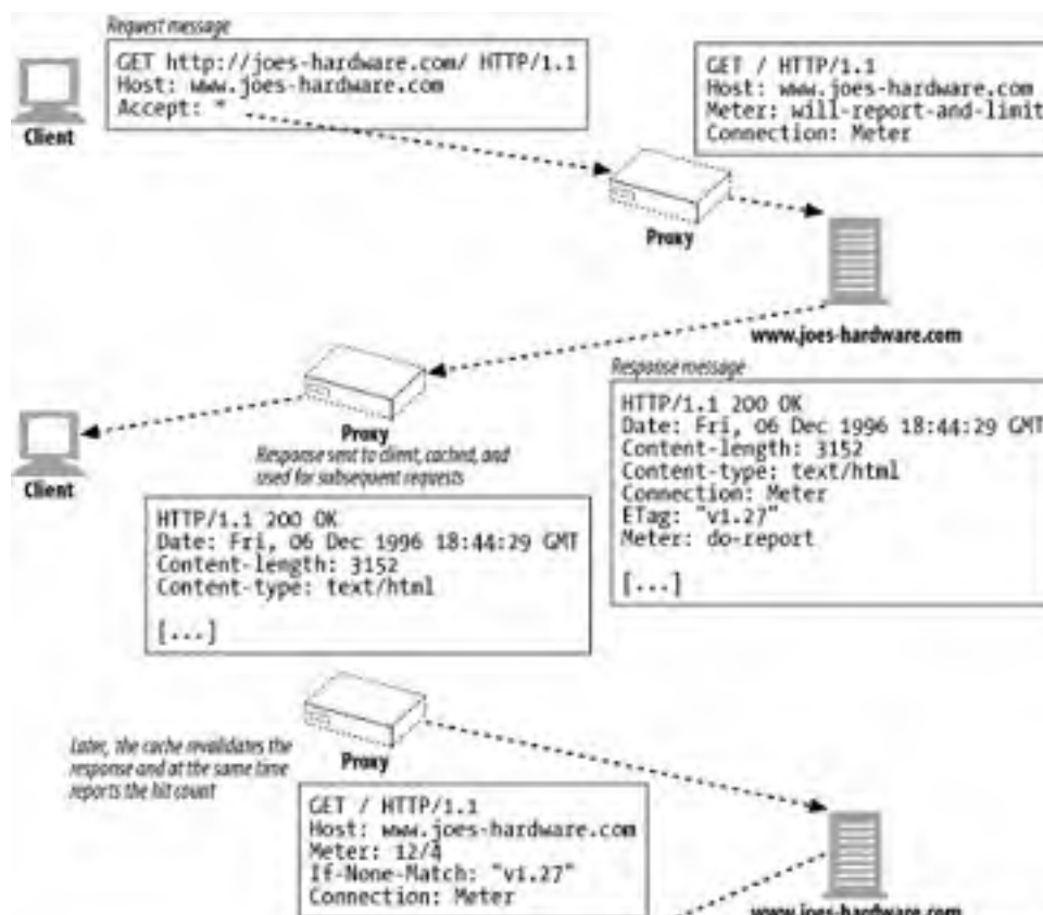
Figure 21-1. Hit Metering example
