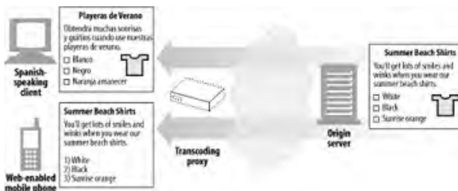
Anonymizer (Figure 6-10)
