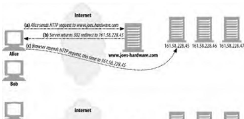
Figure 20-1. HTTP redirection
