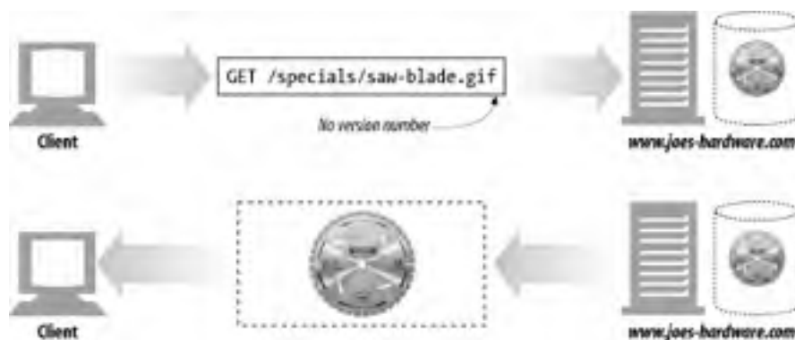
Figure 3-6. HTTP/0.9 transaction
