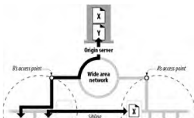
Figure 7-10. Sibling caches
