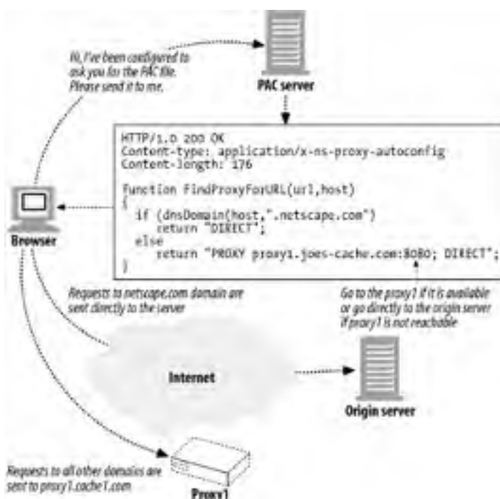
Figure 20-10. Proxy auto-configuration
