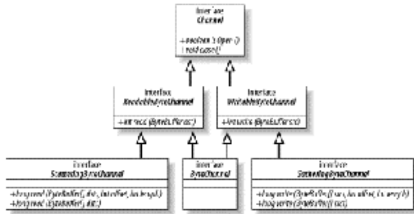
Figure 3-4. Scatter/gather interfaces
