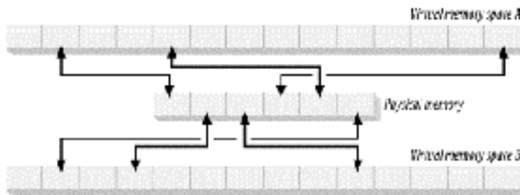
Figure 1-4. Memory pages
