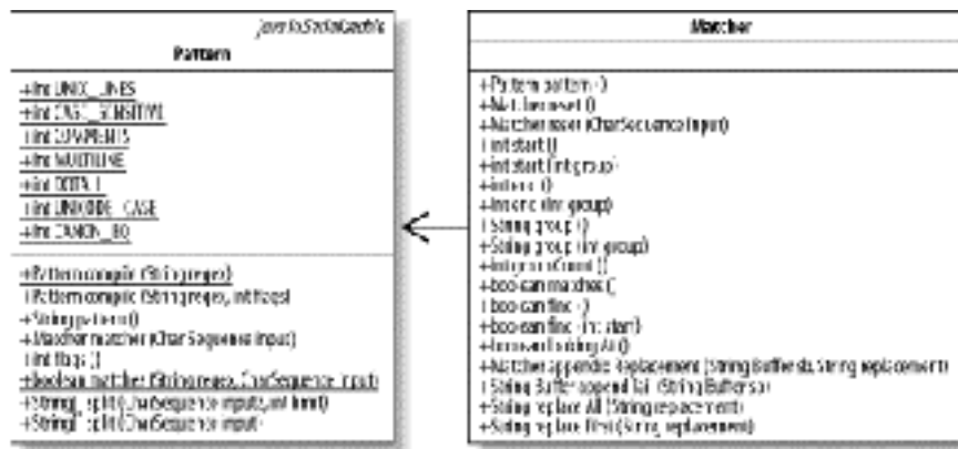
Figure 5-1. The regular expression classes
