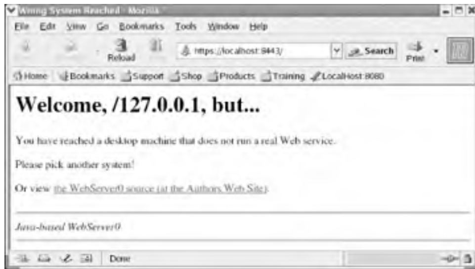
Figure 17-2. With encryption
