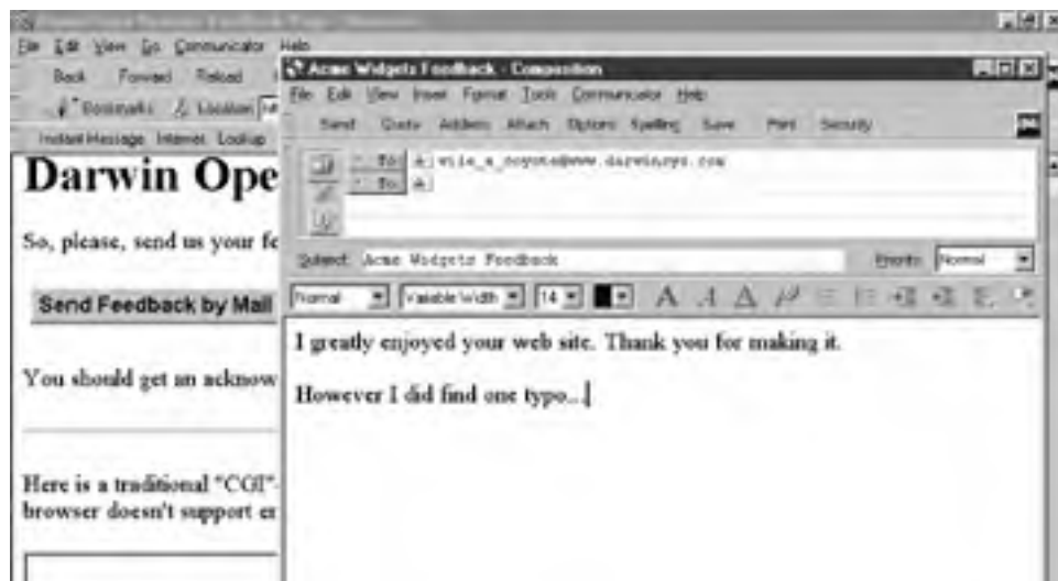
Figure 19-1. MailtoButton
