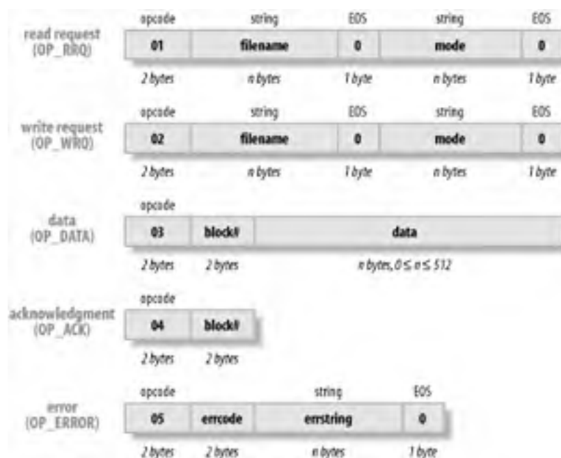
Figure 16-1. The TFTP protocol packet formats
