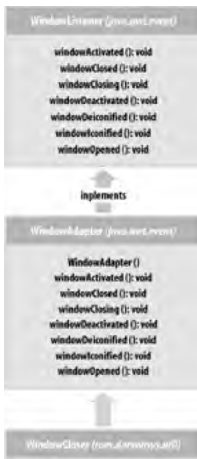
Figure 14-5. WindowListener, WindowAdapter, and my WindowCloser
