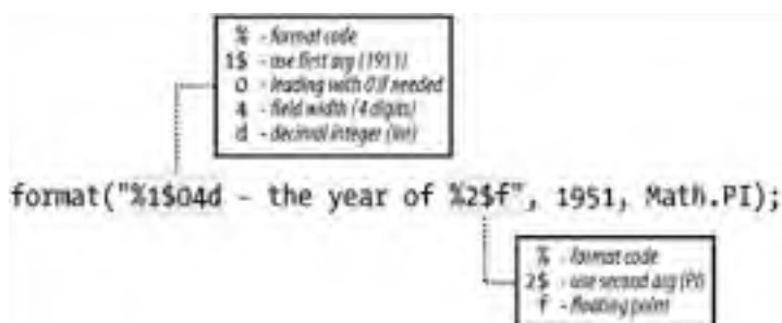
Figure 10-2. Format codes examined
