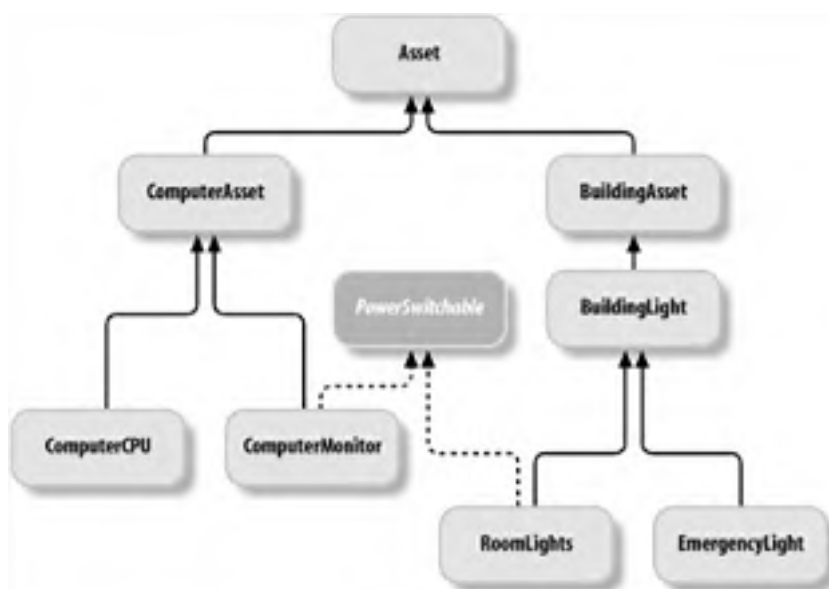
Figure 9-1. Classes for a building management system
