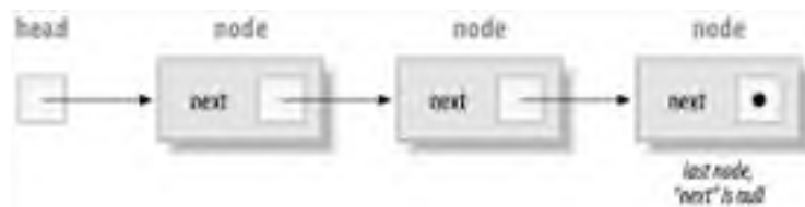
Figure 7-1. Linked list structure
