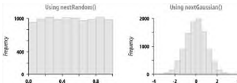
Figure 5-1. Flat (left) and Gaussian (right) distributions
