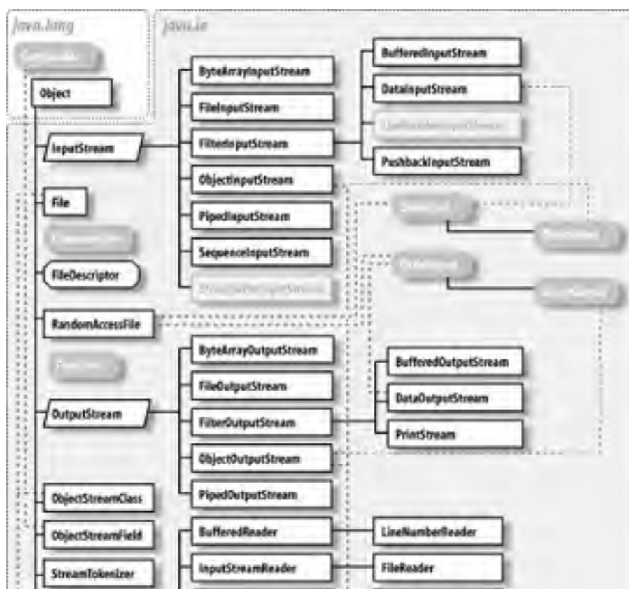
Figure 10-1. java.io classes
