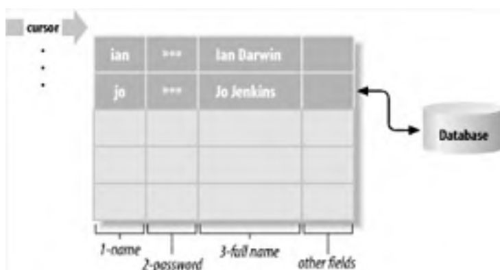
Figure 20-1. ResultSet illustrated
