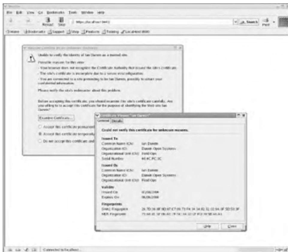
Figure 17-1. Browser caution
