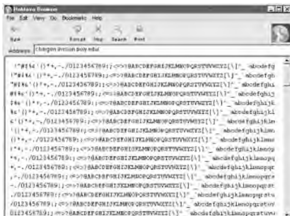
Figure 16-3. HotJava using the chargen protocol handler
