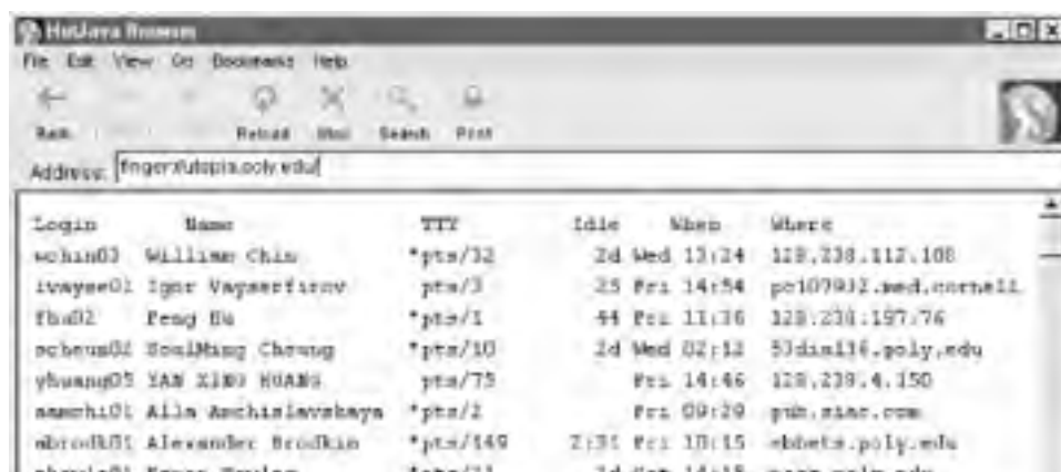
Figure 16-1. HotJava using the finger protocol handler
