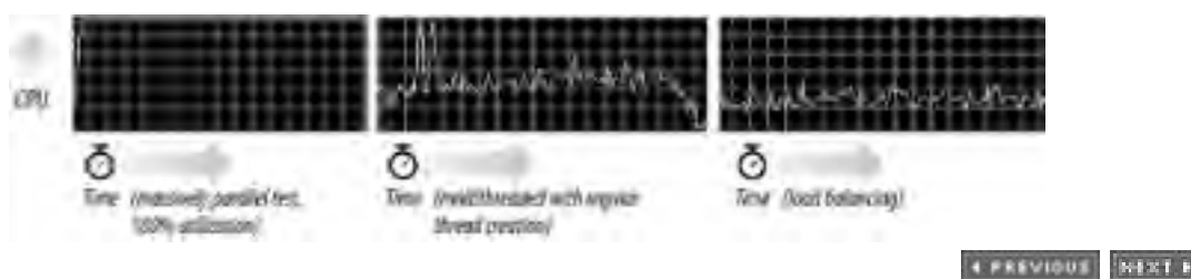
Figure 10-5. CPU utilization for various download tests
