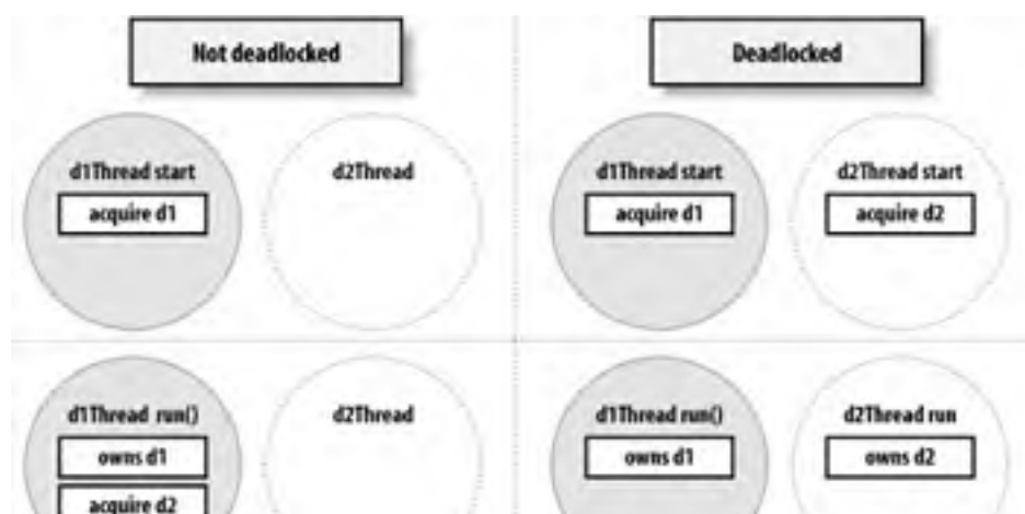
Figure 10-2. The difference between nondeadlocked and deadlocked execution
