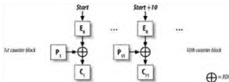
Figure 5-4. Counter (CTR) mode
