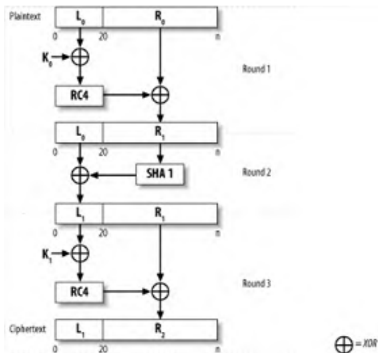
Figure 5-6. The structure of LION
