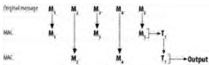
Figure 6-8. Properly interleaving MACs
