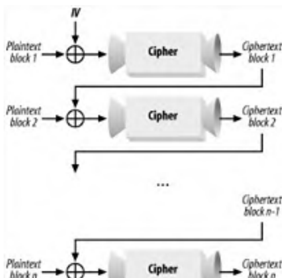
Figure 5-1. CBC mode
