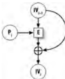
Figure 6-1. The Davies-Meyer construct
