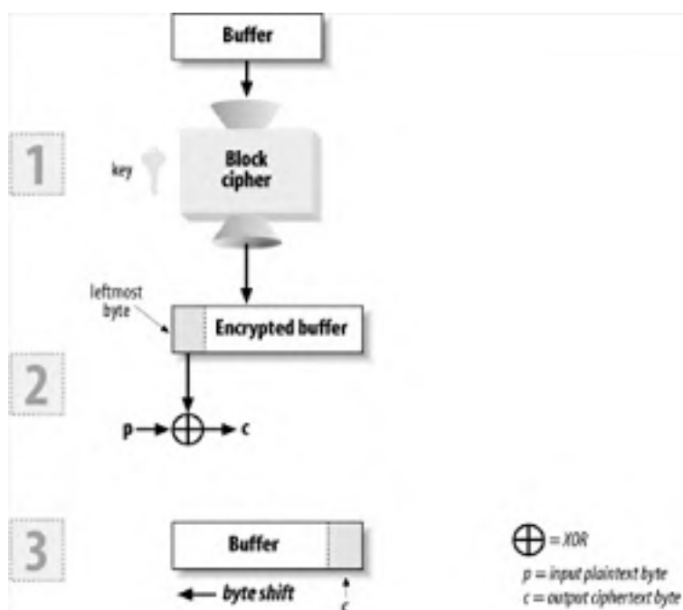
Figure 5-2. CFB mode
