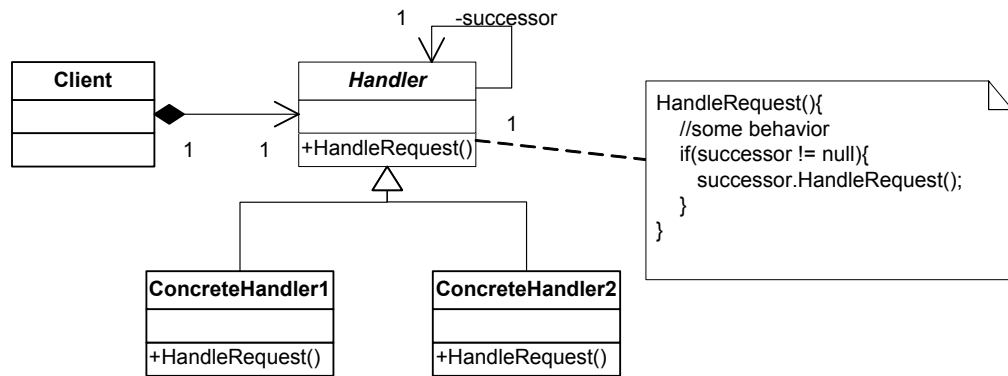
Figure 14-3: The Chain of Responsibility design pattern
