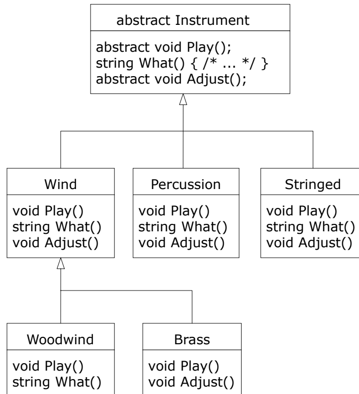
Figure 8-4: Abstract classes provide shared behavior, but cannot be instantiated Here's the orchestra example modified to use abstract classes and methods:
