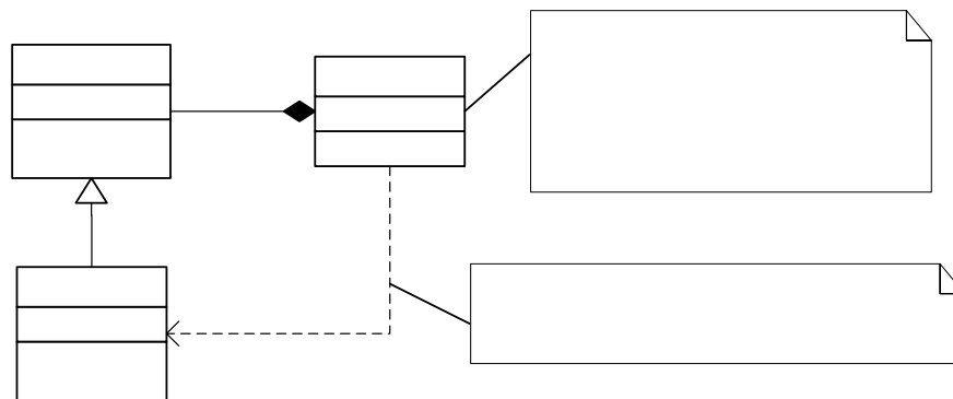
Figure 7-3: Late binding can cause undesired behavior if the base type changes
