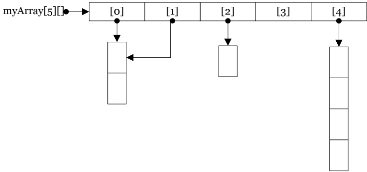
Figure 5-1: Jagged arrays can have complex relationships to physical memory. A rectangular array, on the other hand, is a contiguous block:
