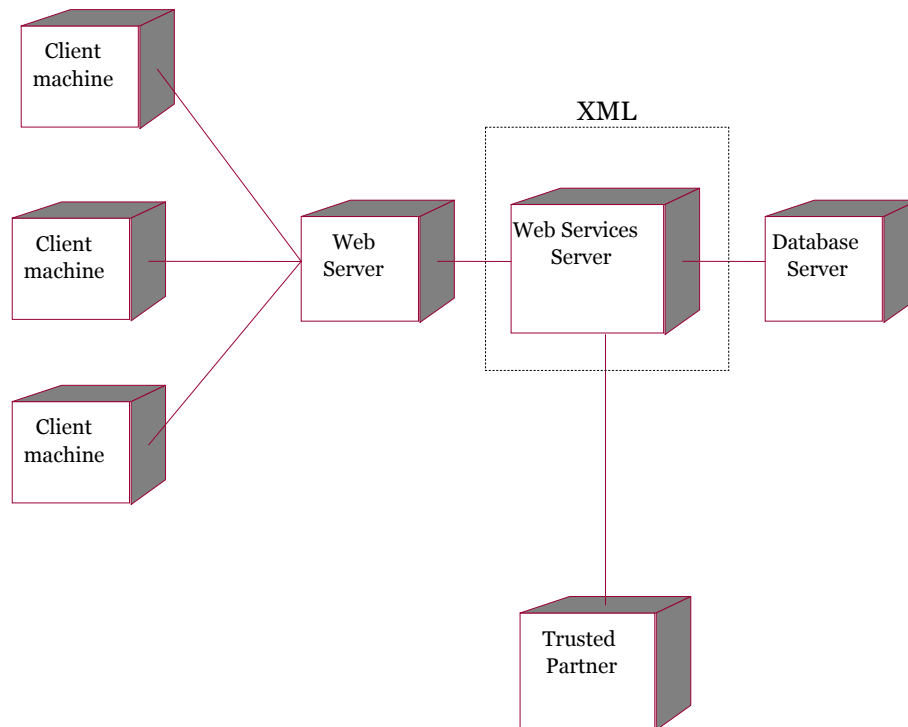
Figure 18-4: Not all server-side programming is Web Service programming
