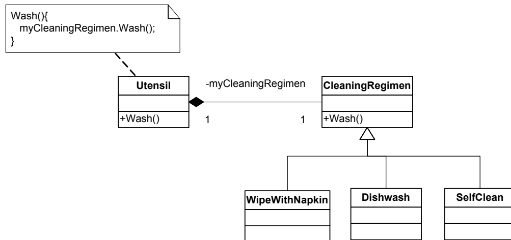
Figure 7-6: The Strategy design pattern
