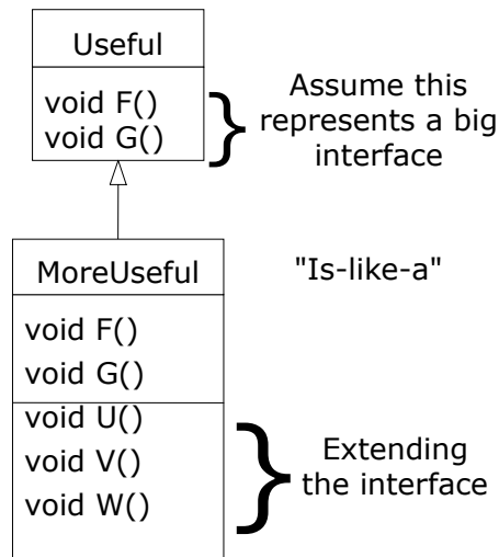
Figure 8-7: The subtype extends the base class
