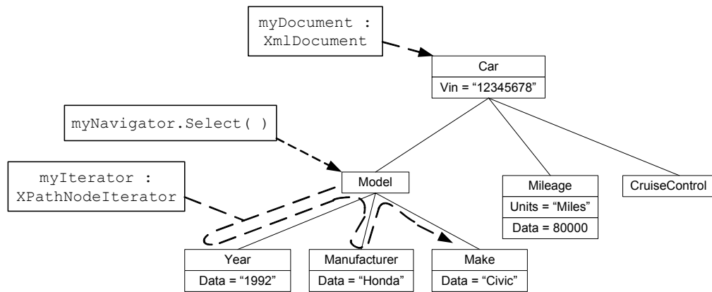
Figure 17-4: Navigating with XPathNodeIterator
