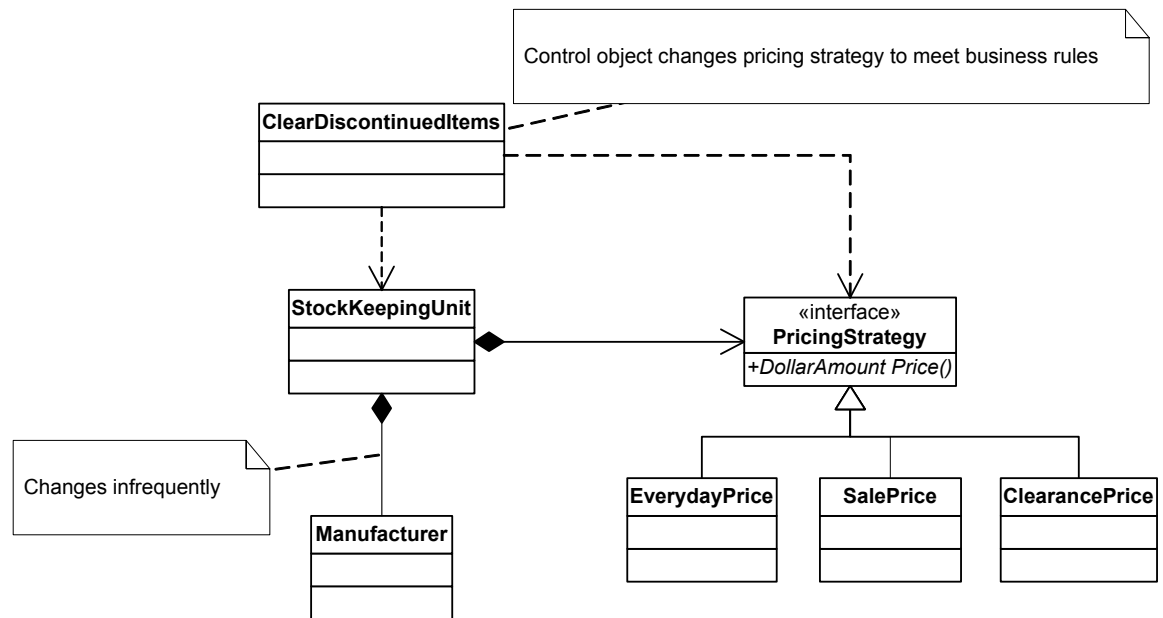
Figure 9-1: Not all objects correspond to “physical things in the real world.”
