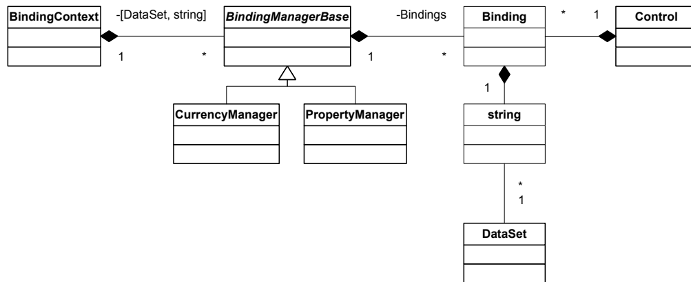
Figure 14-11: Coordinating the relationship between Controls and DataSets
