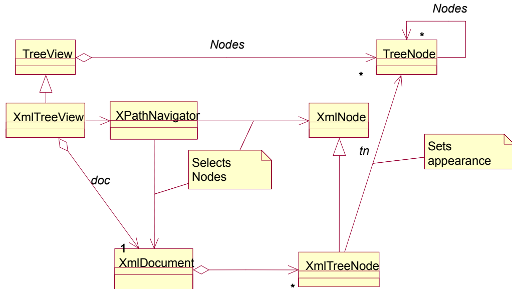
Figure 17-5: The class structure of XmlTreeView
