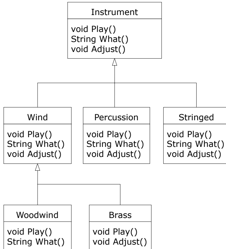
Figure 8-2: Despite increased complexity, old code works
