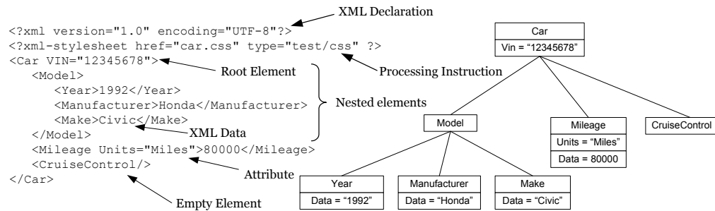
Figure 17-1: An XML document can be viewed as a tree-like data structure
