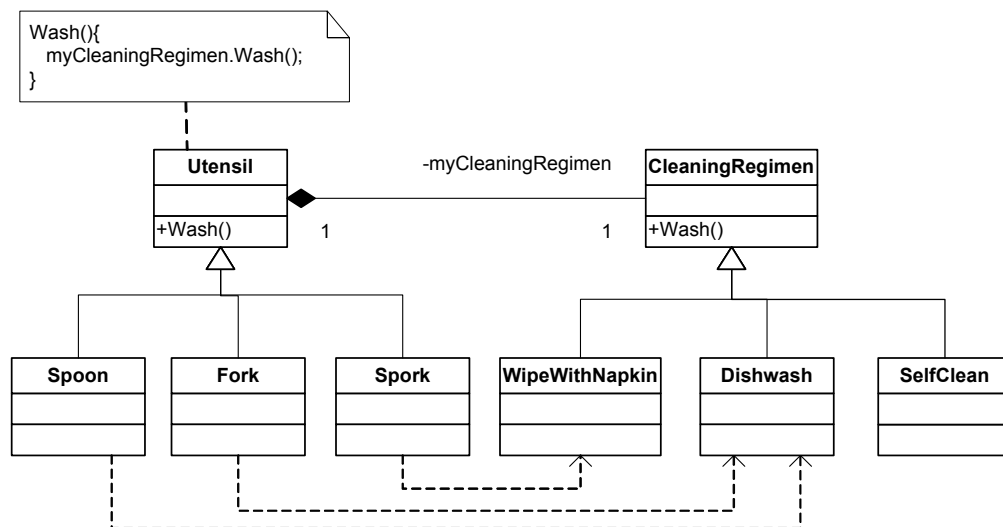
Figure 7-7: Manipulating CleaningRegimens on a per-Utensil basis
