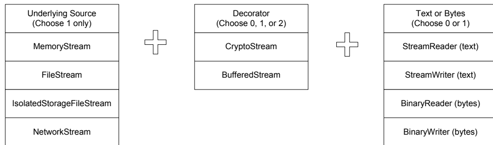
Figure 12-1: Streams use the Decorator pattern to build up capability
