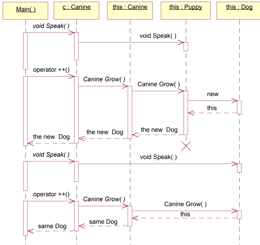
Figure 8-3: Virtual calls to Canine.Grow() and Speak()
