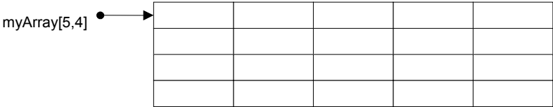
Figure 5-2: Rectangular arrays are contiguous blocks of memory. As you can see from Figures 5-1 and 5-2, jagged arrays are best thought of as “references to references” while a rectangular array can be safely thought of as a
