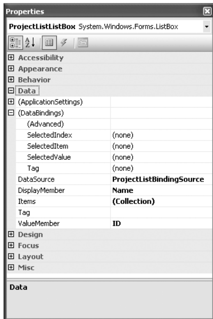
Figure 9-13. Data properties for the ListBox control
