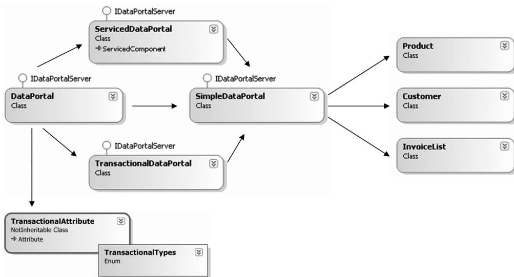
Figure 4-4. Types supporting transactional technologies in the data portal
