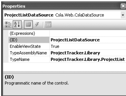
Figure 10-17. Properties for the ProjectListDataSource control
