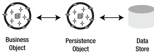
Figure 2-7. Separation of ORM logic into a persistence object
