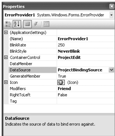
Figure 9-22. Properties for the ErrorProvider control
