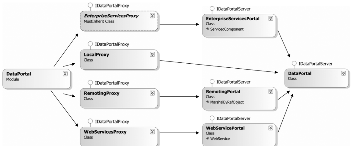
Figure 4-2. Flow of a client call through the data portal
