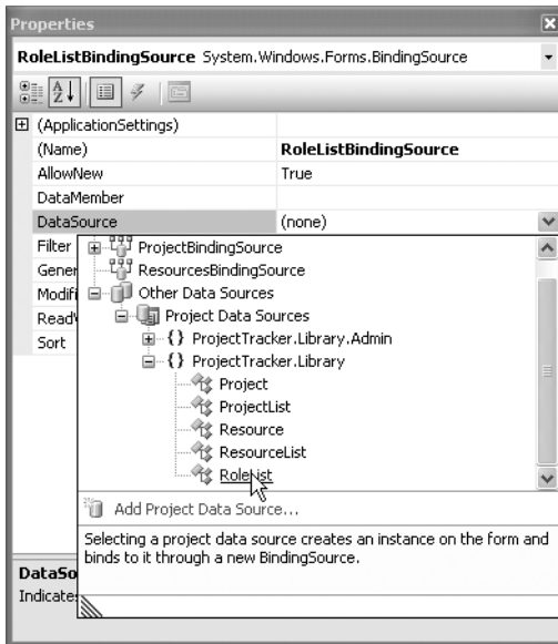
Figure 9-17. Setting the DataSource property on a BindingSource control
