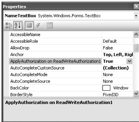
Figure 9-23. ApplyAuthorization property on the NameTextBox control
