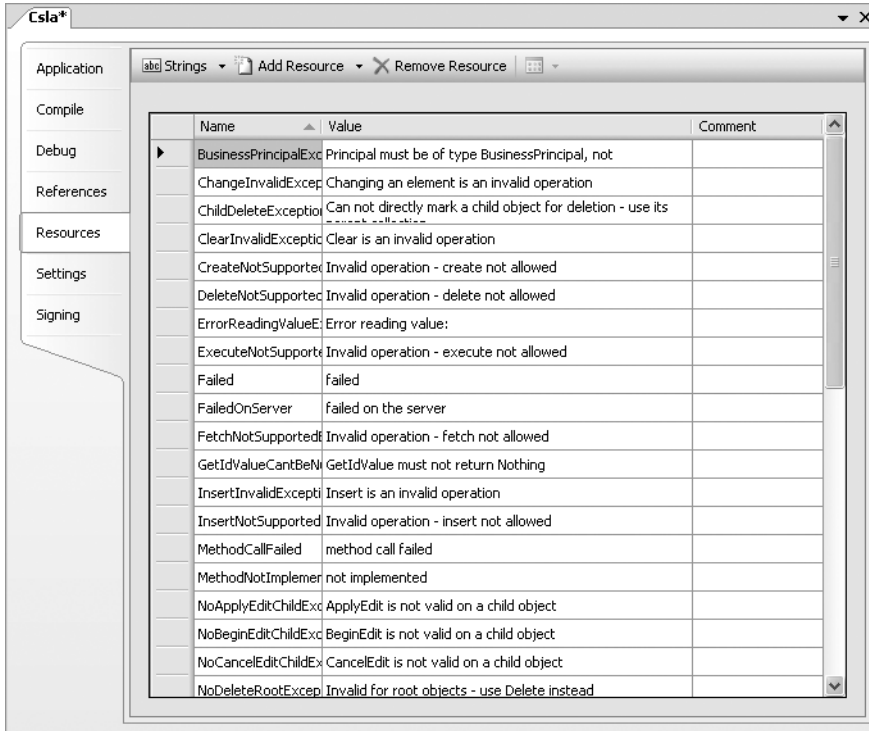
Figure 3-2. Visual Studio resource editor
