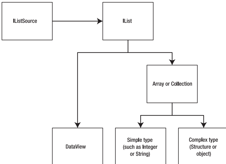
Figure 5-5. Data sources supported by ObjectAdapter
