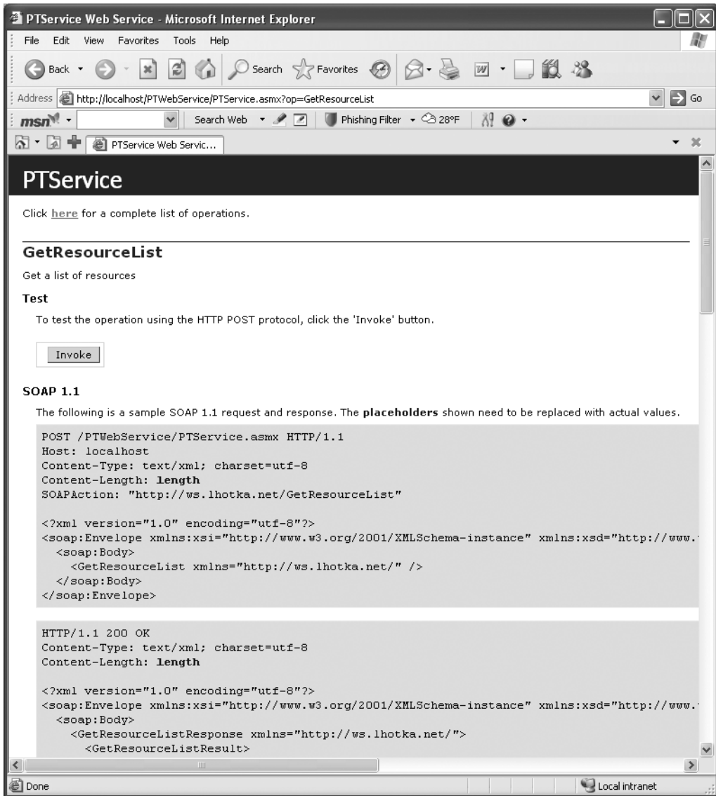
Figure 11-9. WSDL for the GetResourceList web method
