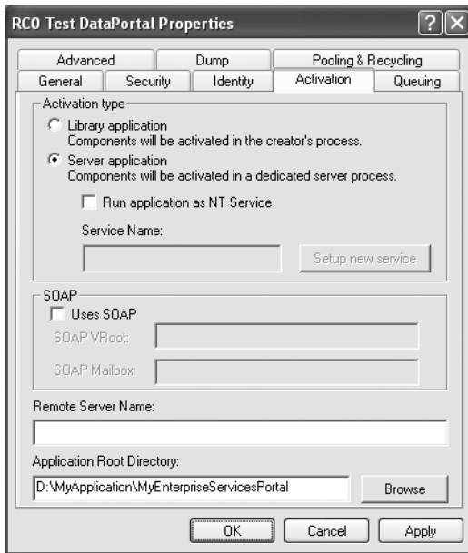
Figure 4-10. Setting the application root directory
