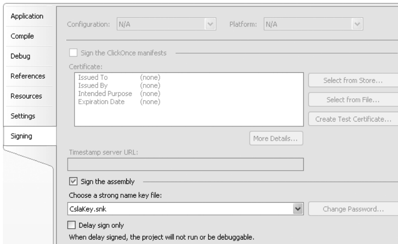
Figure 4-9. Signing an assembly using the Project Properties designer
