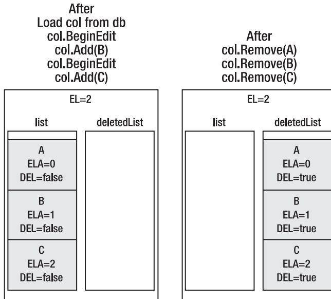
Figure 3-6. A more complex example with nested edit method calls
