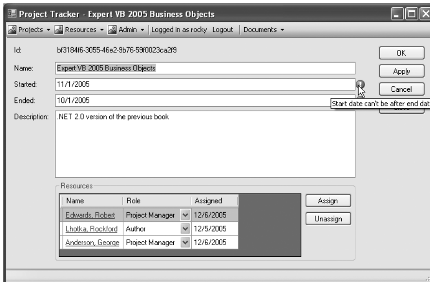
Figure 9-21. The ErrorProvider control displaying validation error information
