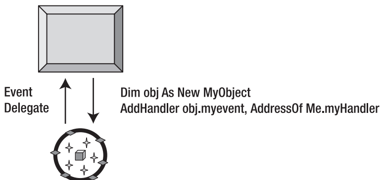
Figure 2-5. Handling an event on an object causes a back reference to the form.
