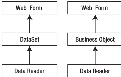
Figure 10-3. Data loaded into an intermediate object, followed by the web form
