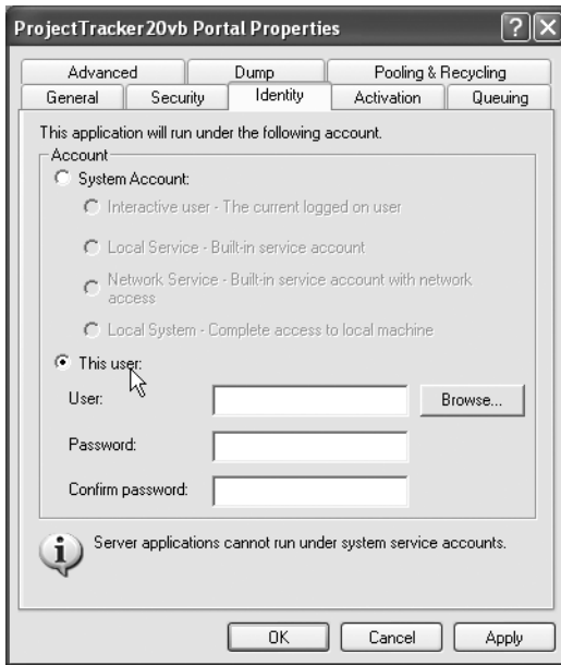
Figure 12-7. Setting the identity account for the service
