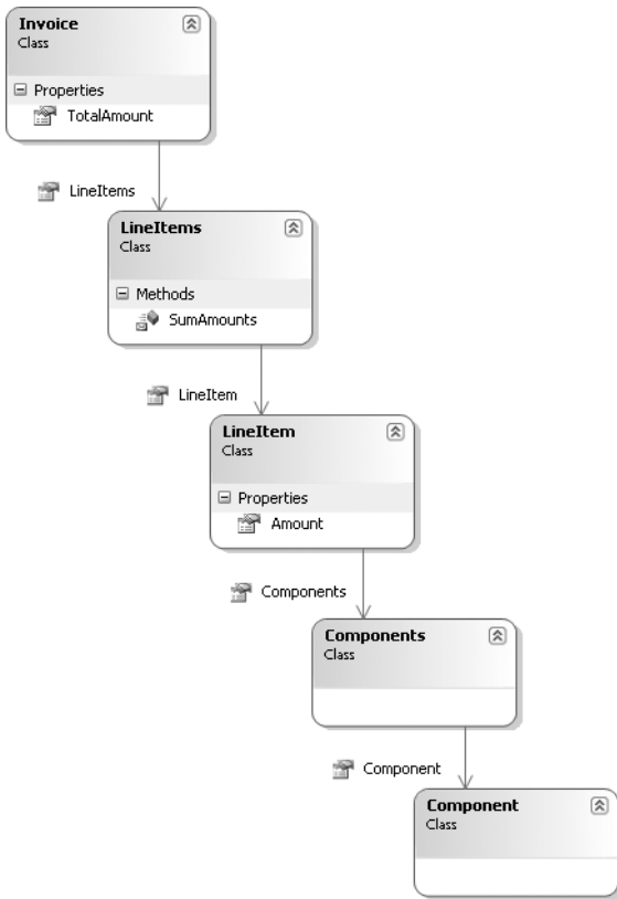
Figure 2-3. Class diagram showing a more complex set of class relationships
