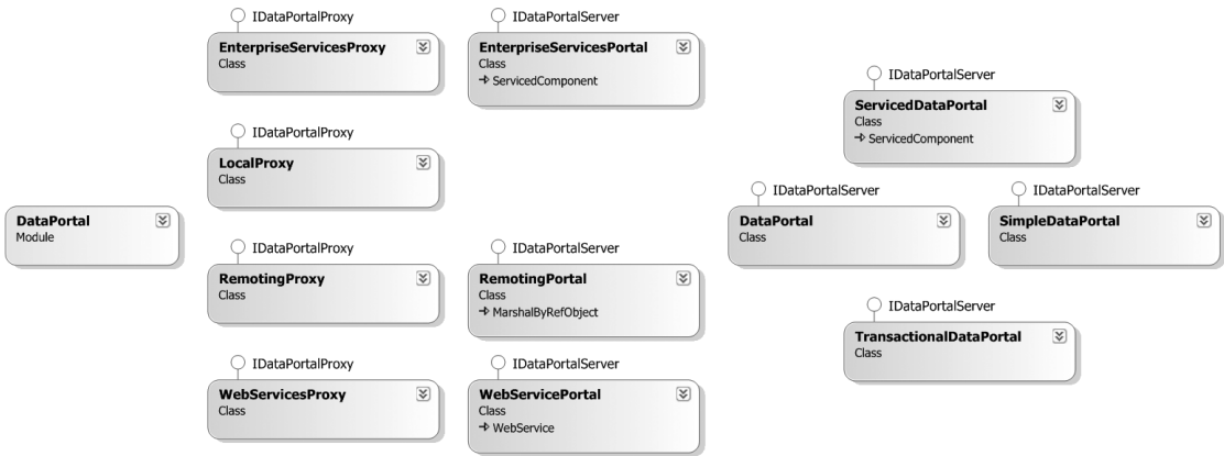
Figure 4-1. Types required to implement data access, mobile objects, and security
