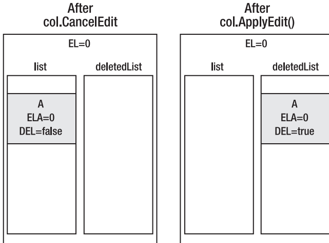
Figure 3-8. Result after calling either CancelEdit() or ApplyEdit()
