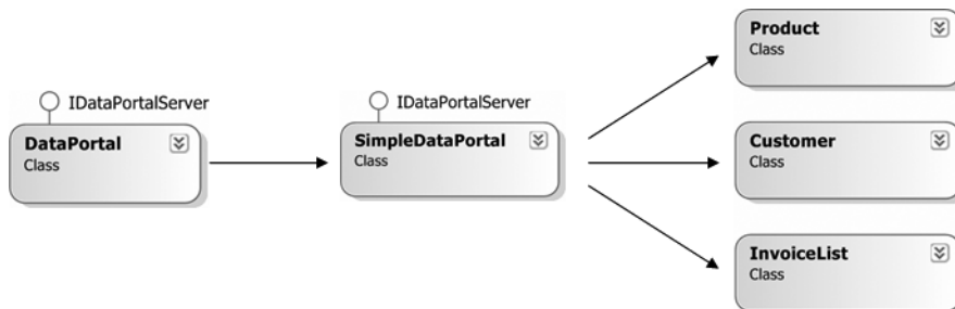
Figure 4-3. Flow of a client call through the message router
