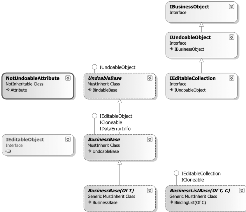
Figure 2-11. Separating n-level undo into Core.UndoableBase
