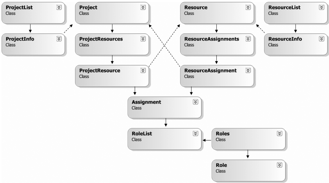
Figure 8-1. ProjectTracker application classes
