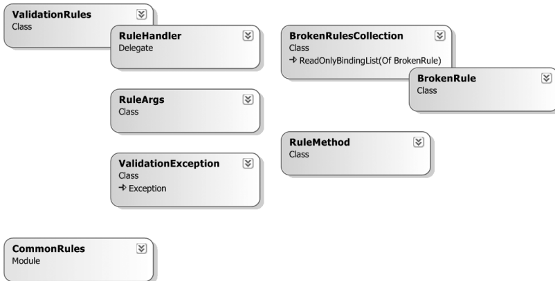
Figure 2-13. Classes implementing the validation rules behavior
