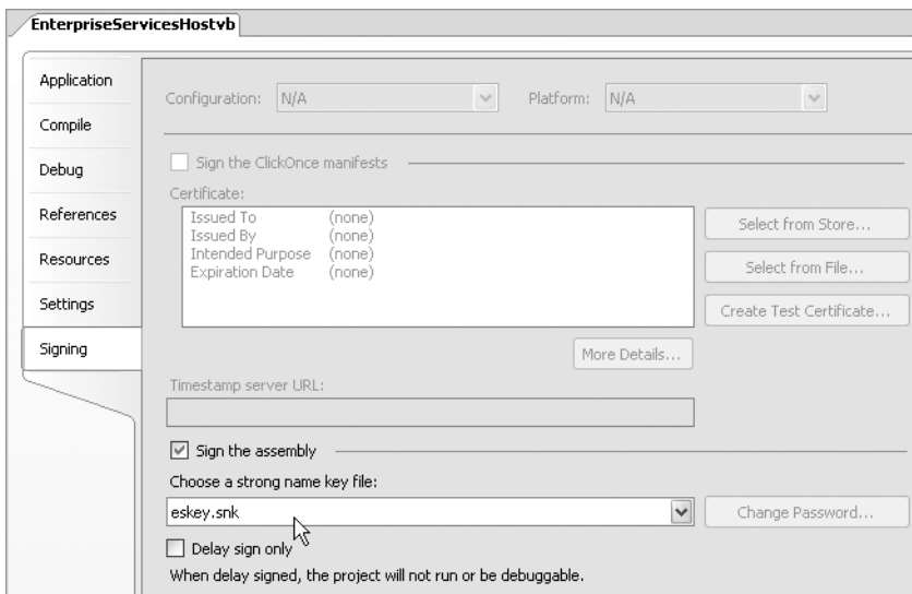
Figure 12-5. Signing the assembly
