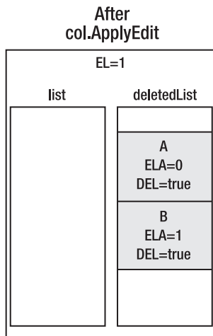
Figure 3-7. The result after calling ApplyEdit()
