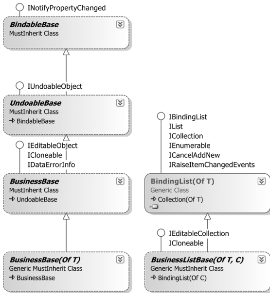
Figure 2-12. Class diagram with BindableBase and BindingList(Of T)
