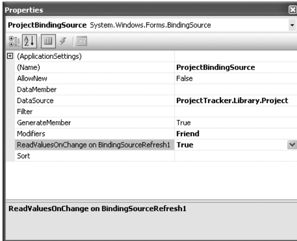
Figure 9-24. The ReadValuesOnChange property on the ProjectBindingSource control
