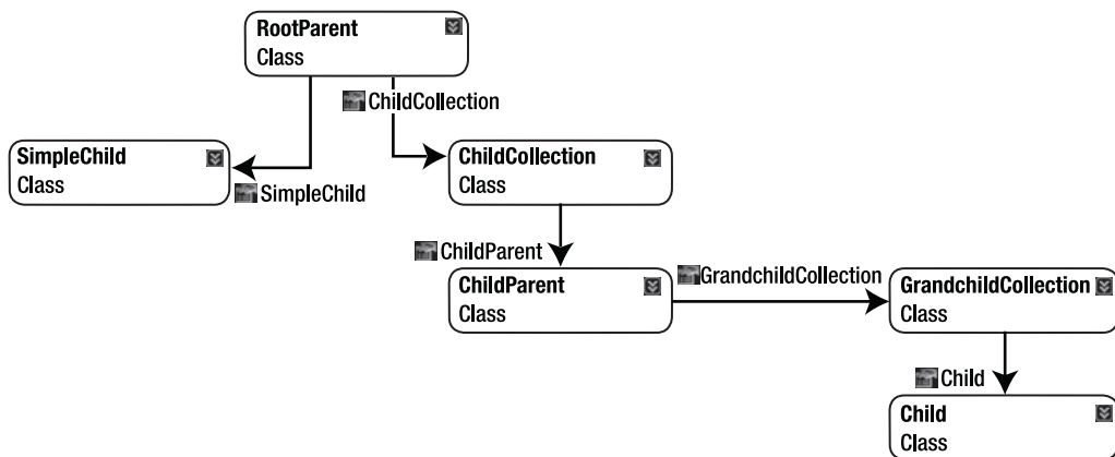
Figure 3-3. Class diagram showing how root, child, and grandchild objects are related
