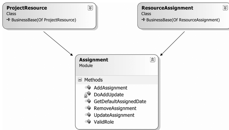
Figure 8-4. Objects collaborating with Assignment
