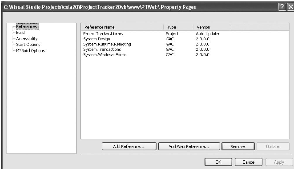
Figure 10-8. Referencing ProjectTracker.Library
