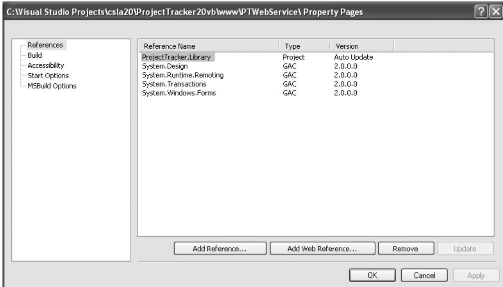
Figure 11-7. Referencing ProjectTracker.Library
