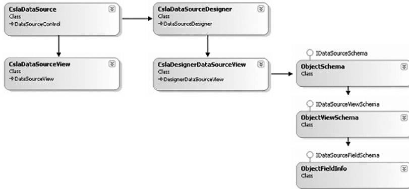
Figure 5-7. Relationship between the classes in CslaDataSource
