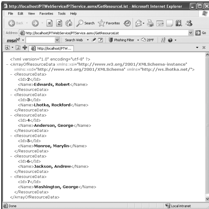
Figure 11-10. Results of invoking the GetResourceList method
