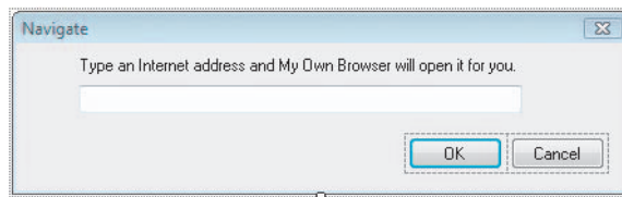
Figure 6-8 Navigate form
