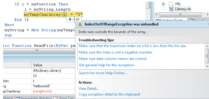
Figure 7-8 Exception Assistant
