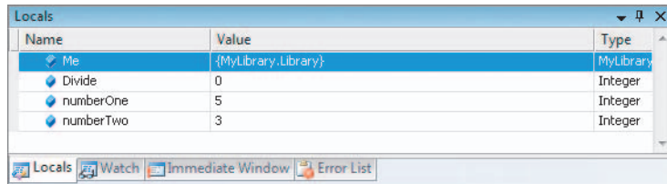
Figure 7-5 Tabs present during debugging in Visual Studio
