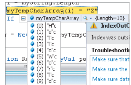
Figure 7-9 Array visualizer
