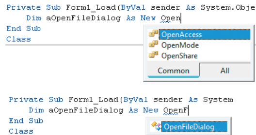
Figure 5-6 IntelliSense narrows down the options based on the context.
