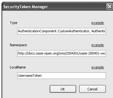
Figure 33-12. Configuring a new UsernameTokenManager
