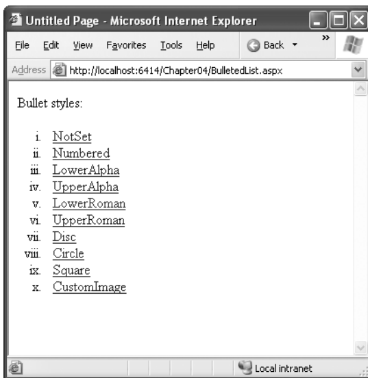
Figure 4-11. Different BulletedList styles
