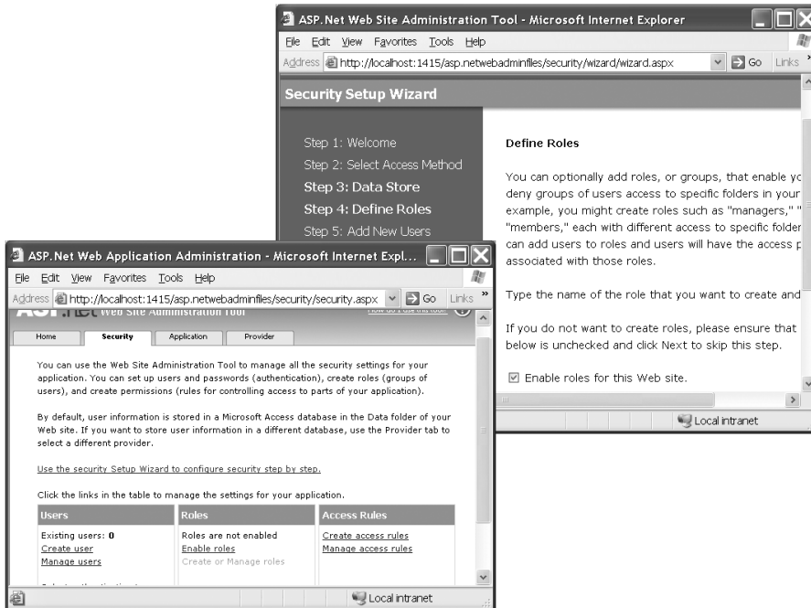
Figure 23-2. Configuring the roles service
