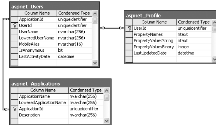
Figure 24-1. The profile tables
