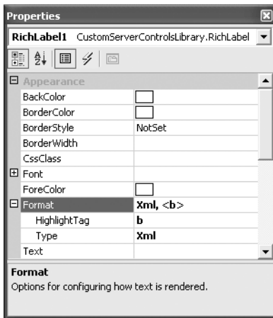
Figure 28-6. Editing properties of the RichLabelFormattingOptions object
