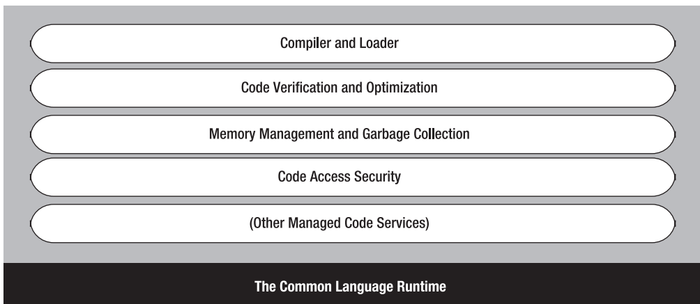
Figure 1-2. The CLR and .NET Framework
