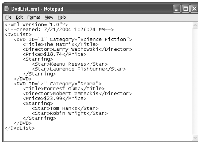
Figure 12-1. A dynamically created XML document
