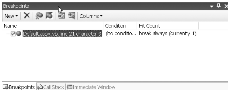
Figure 2-25. The Breakpoints window
