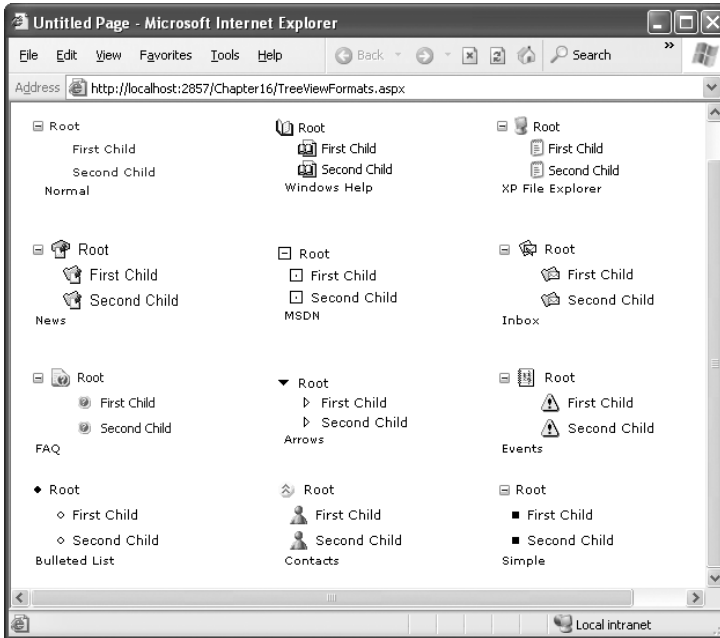
Figure 16-18. Different looks for a TreeView
