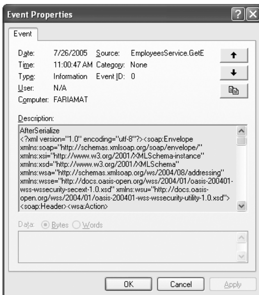
Figure 33-6. A SOAP message in an event log entry
