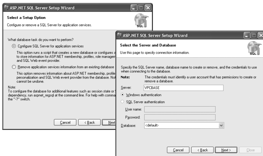
Figure 21-4. The aspnet_regsql.exe wizard user interface
