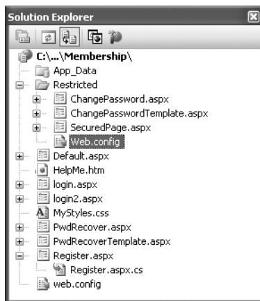
Figure 21-3. The folder and file structure of a web application with a secured area
