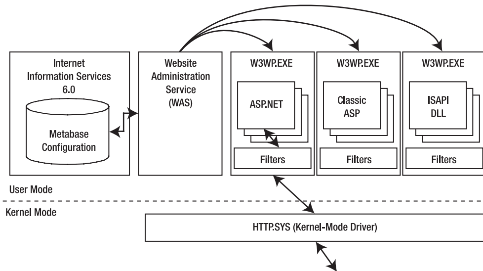
Figure 18-5. The IIS 6.0 process model
