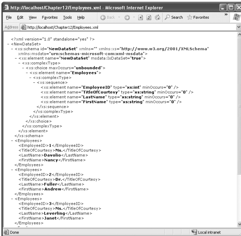
Figure 12-15. Examining the DataSet XML
