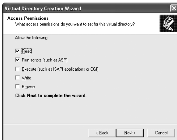
Figure 18-11. Virtual directory permissions
