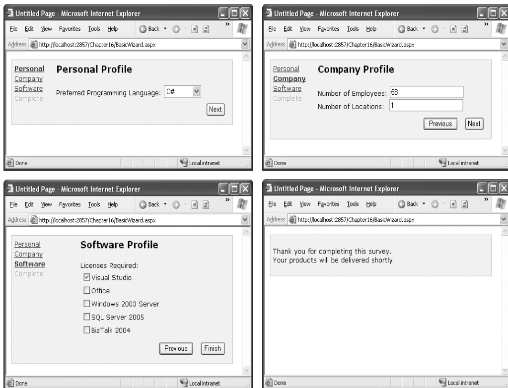
Figure 16-5. A wizard with four steps
