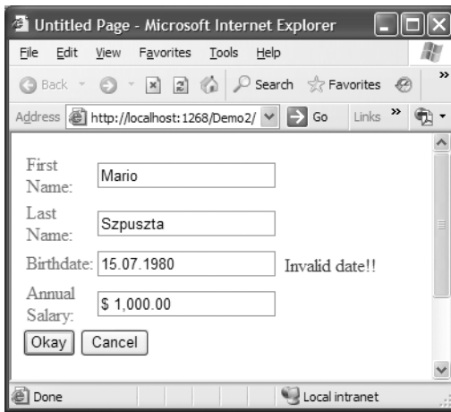
Figure 17-5. Sample application showing localization challenges
