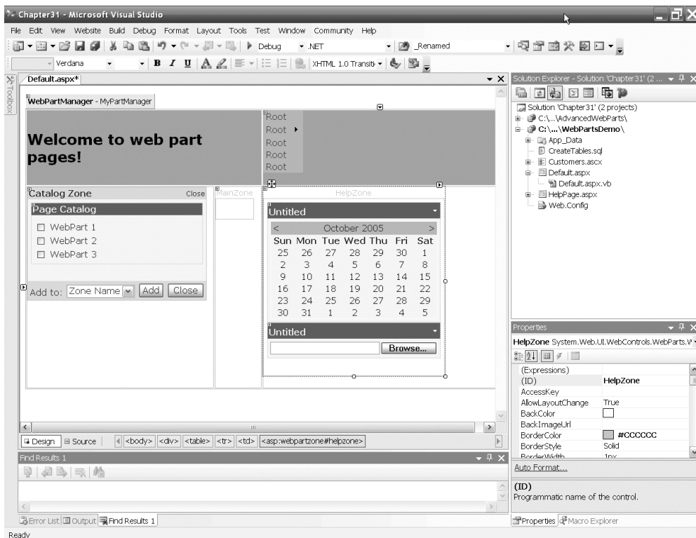
Figure 30-4. A WebPartZone with controls added
