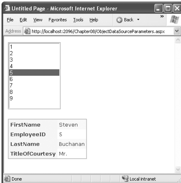
Figure 9-12. Binding to a single employee record
