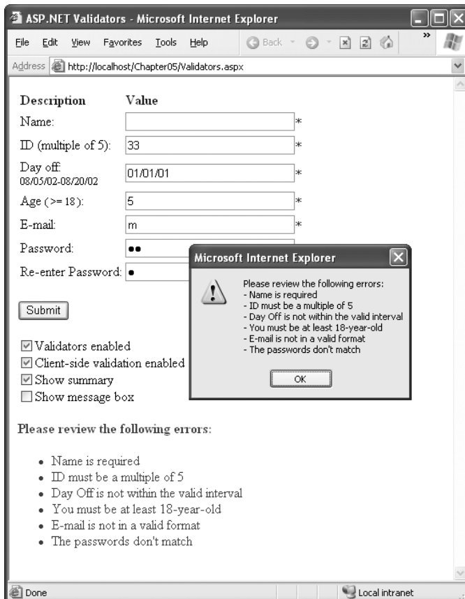
Figure 4-13. The validation summary
