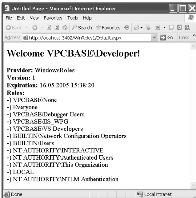
Figure 23-6. Results of querying the RolePrincipal with Windows authentication
