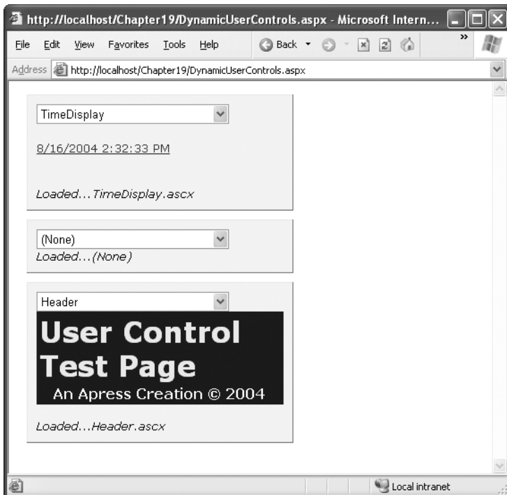
Figure 14-8. A dynamic web page with multiple user controls
