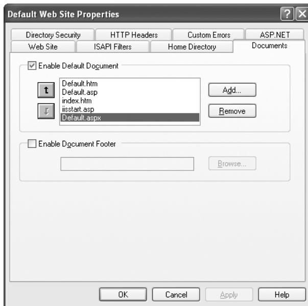
Figure 18-13. The default document list
