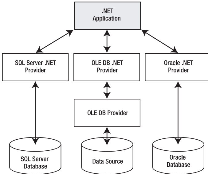
Figure 7-1. The ADO.NET architecture
