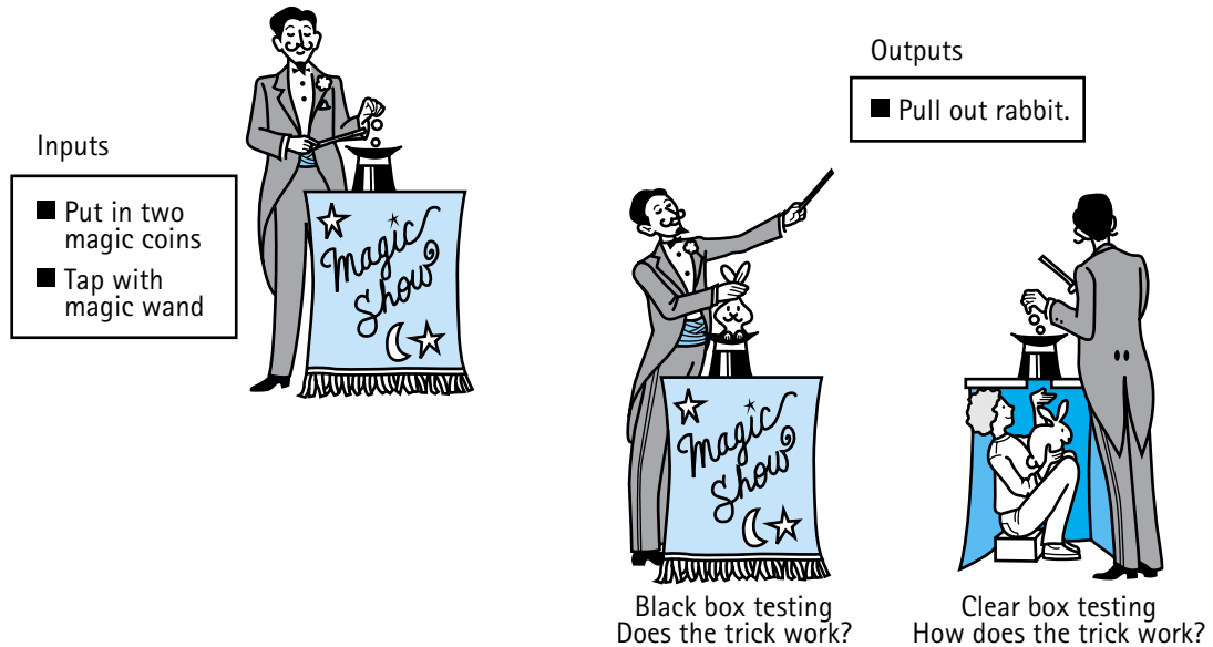
Figure 1.6 Testing approaches
