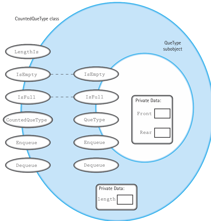
Figure 4.14 Class interface diagram for CountedQueueType class
