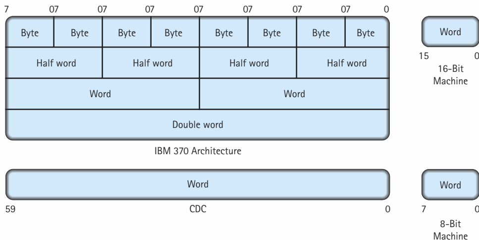
Figure 2.6 Memory configurations
