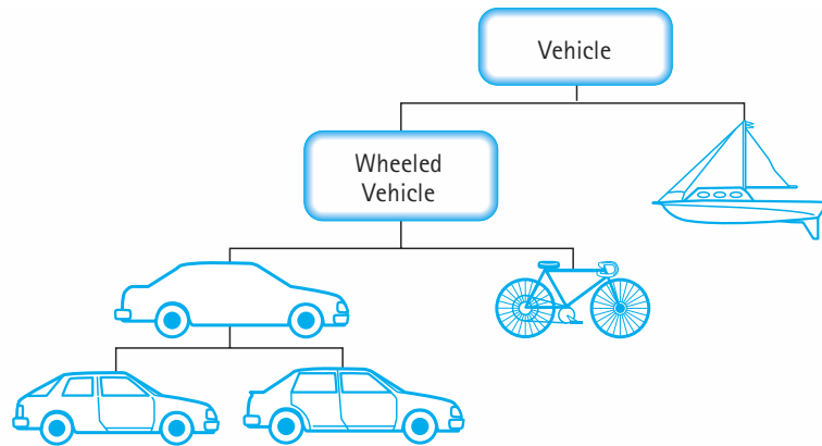
Figure 2.8 Inheritance hierarchy
