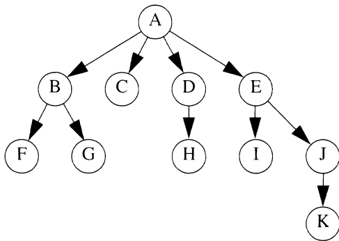
Figure 8.9 A tree.
