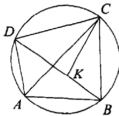
FIGURE 4.3 . Ptolemy's theorem.
