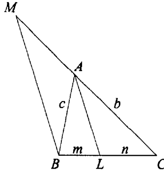
FIGURE 4.20. Angle bisectors.
