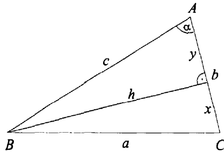
FIGURE 4.2. Proof of the law of cosines.
