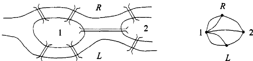
FIGURE 2.6. Königsberg bridges.
