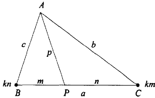
FIGURE 4.13. Another proof of Stewart's theorem.
