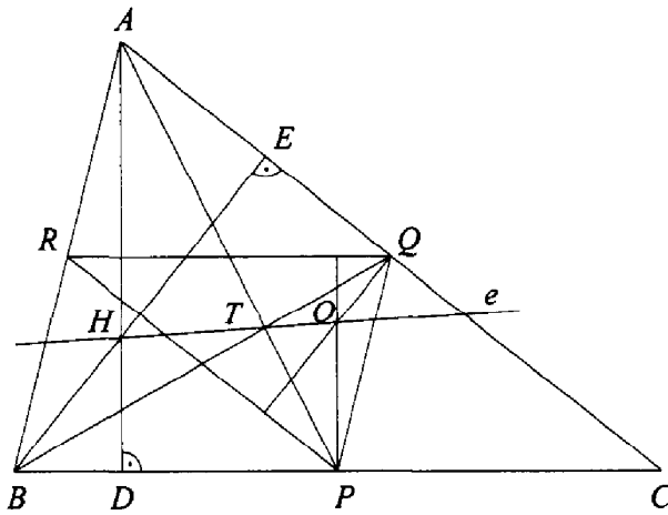
FIGURE 4.14. Euler's line.
