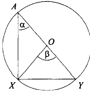
FIGURE 4.4. Central and peripheral angles 1.
