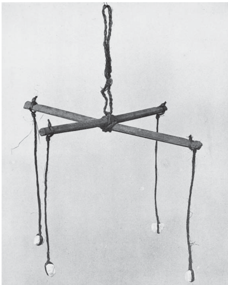
Figure 3.2 A surveying instrument (the plumblines are a modern reconstruction) from the Fayum, dating from Ptolemaic times 13
