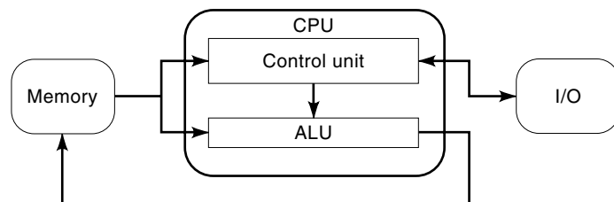
Figure 2. The basic components of a computer with a von Neumann architecture are the memory, which stores both instructions and data, the central processing unit (CPU), which actually executes the instructions, and the input/output (I/O) devices, which provide an interface to the outside world.
