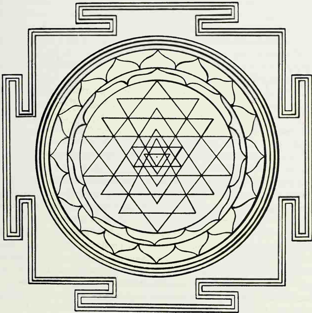
Fig. 4 Shri yantra
